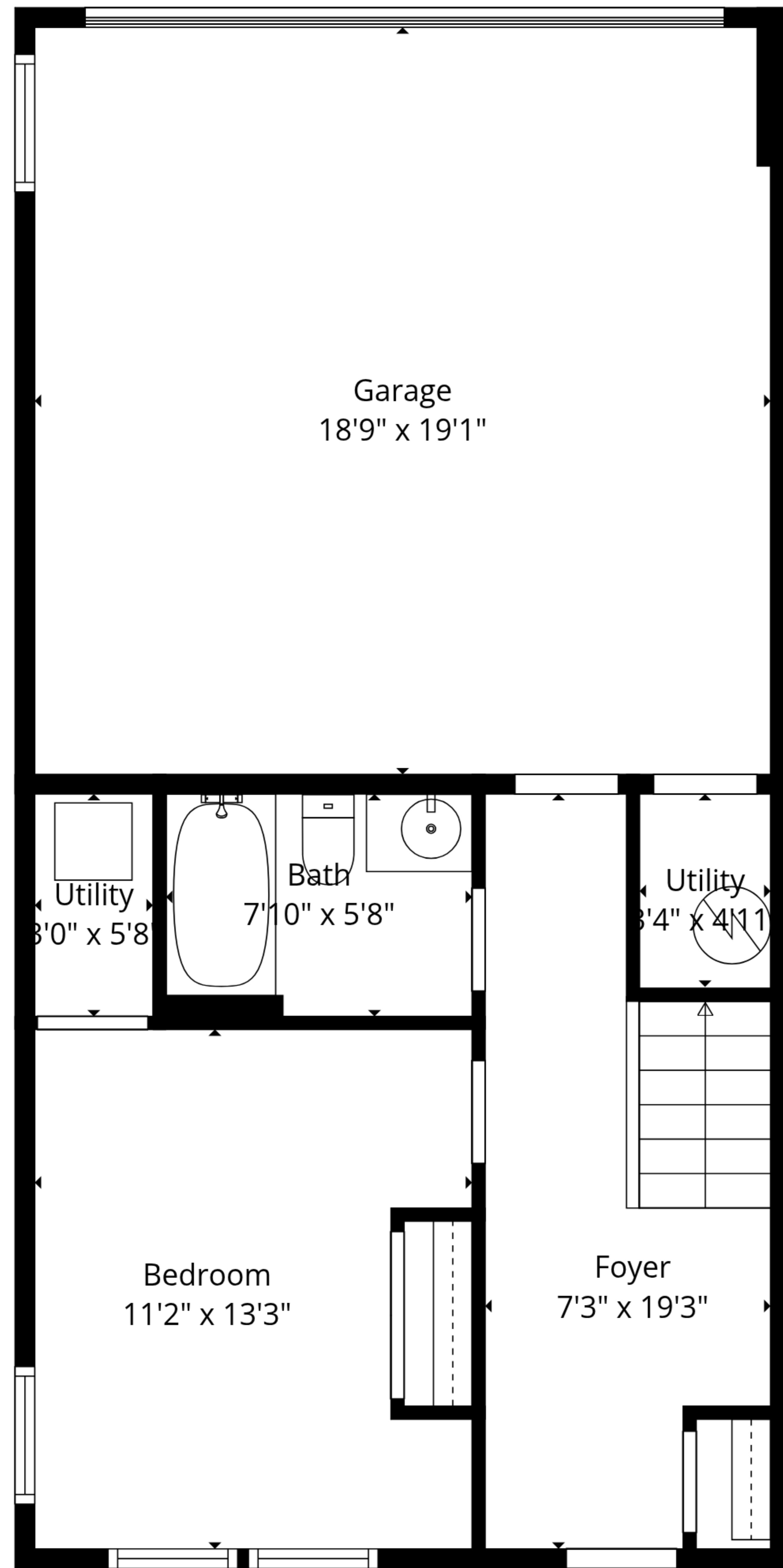
1st Floor
