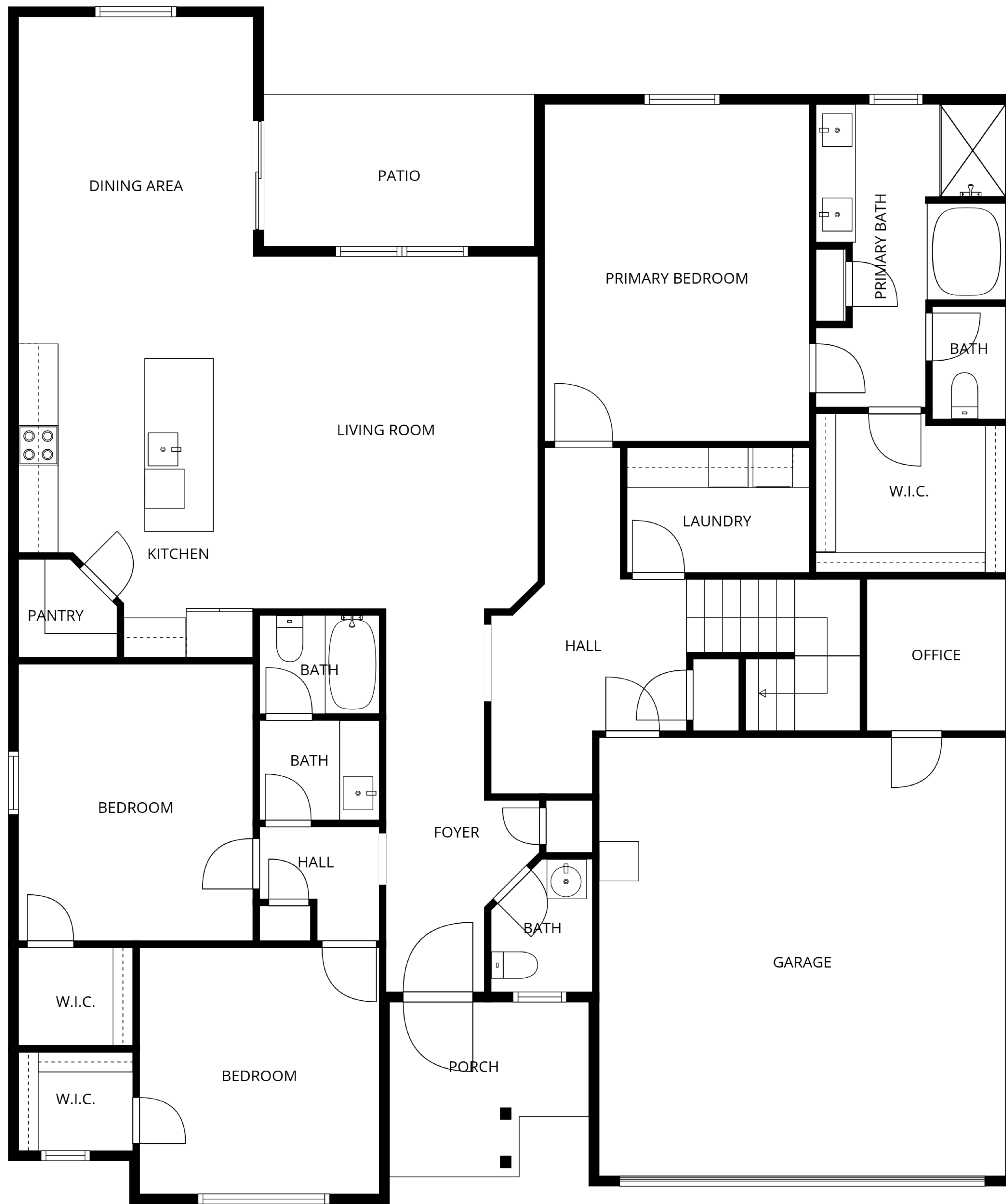
1st floor
