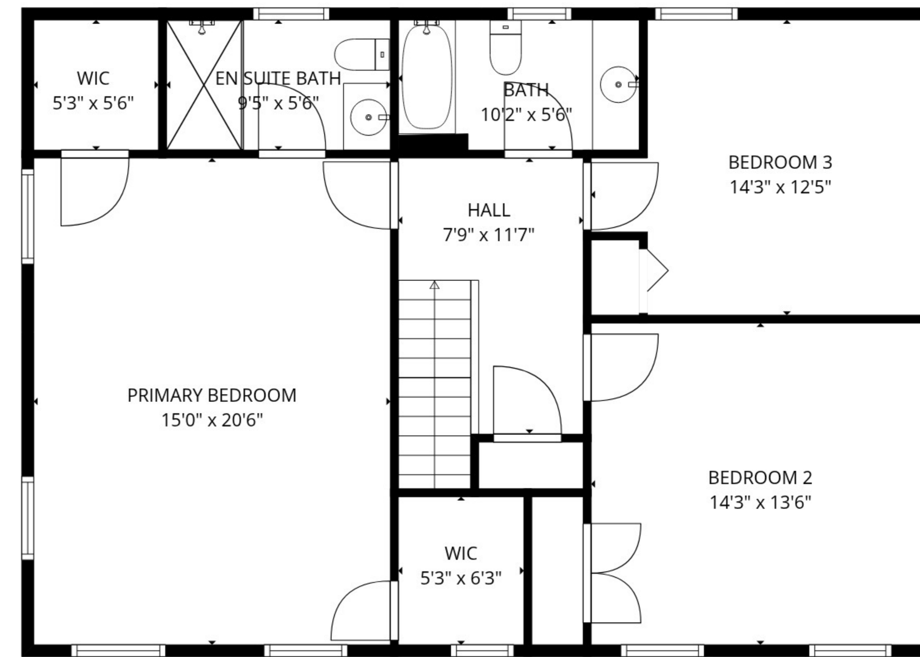
2nd floor
