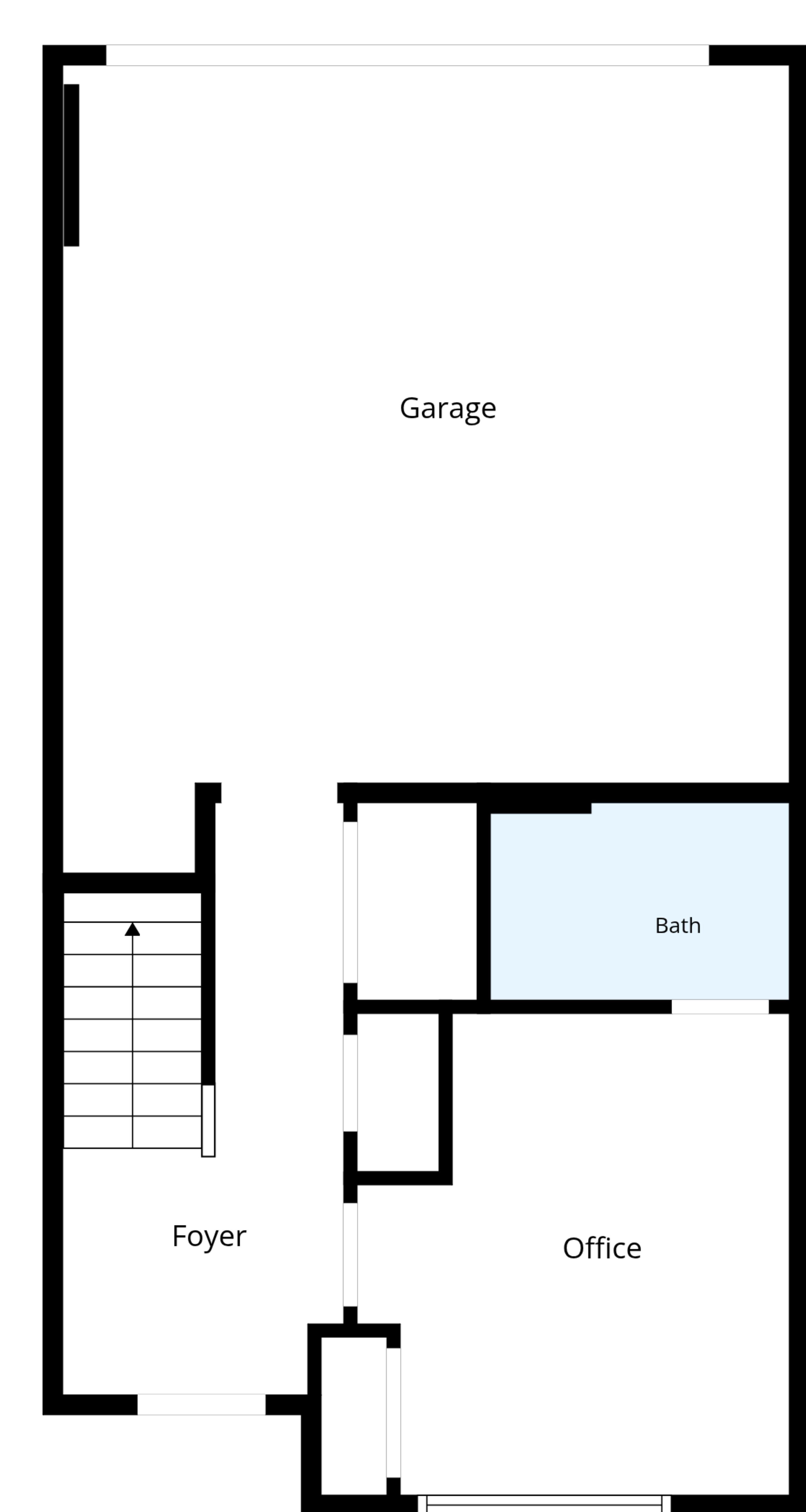
Ground Floor
