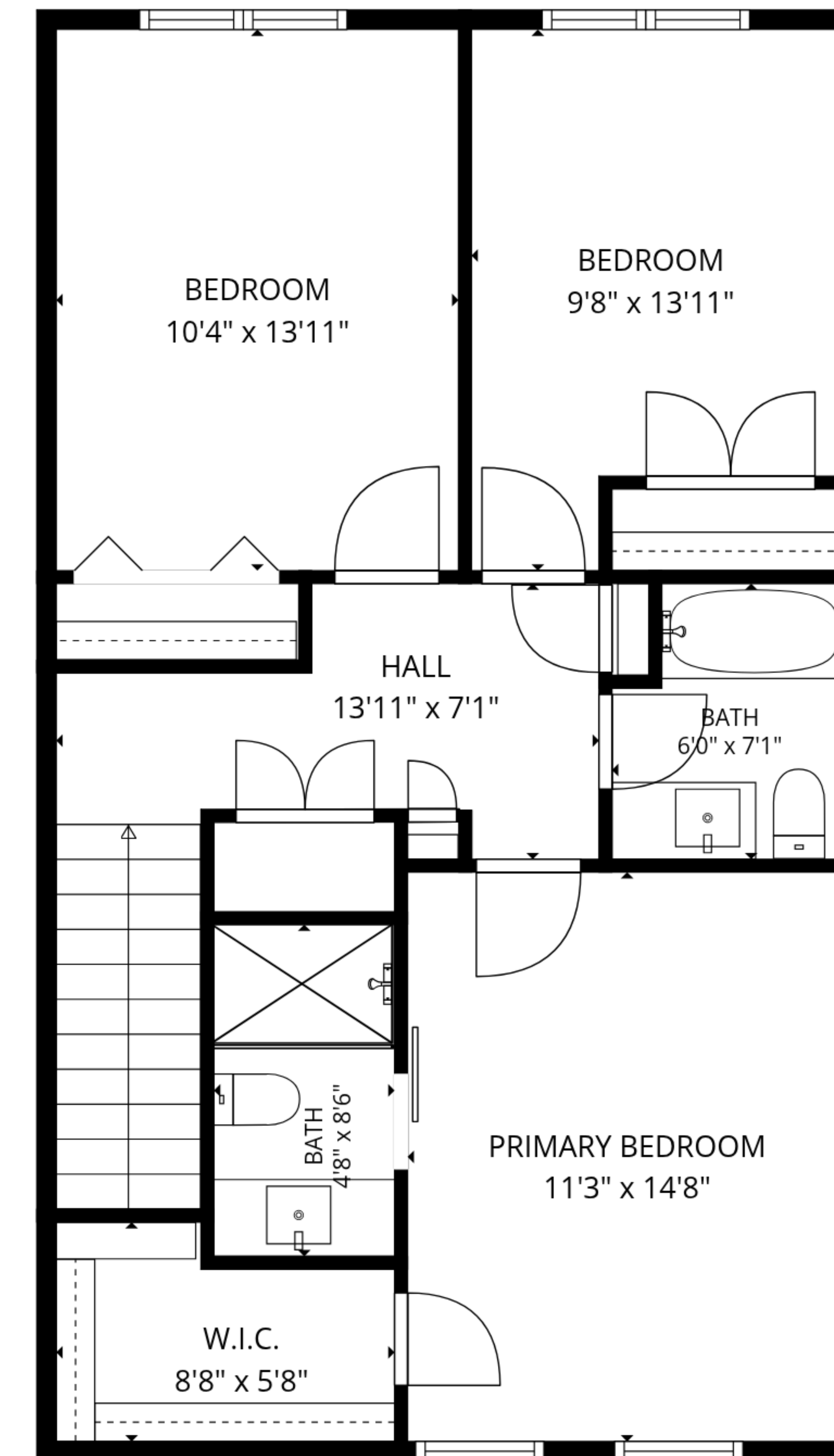
2nd floor
