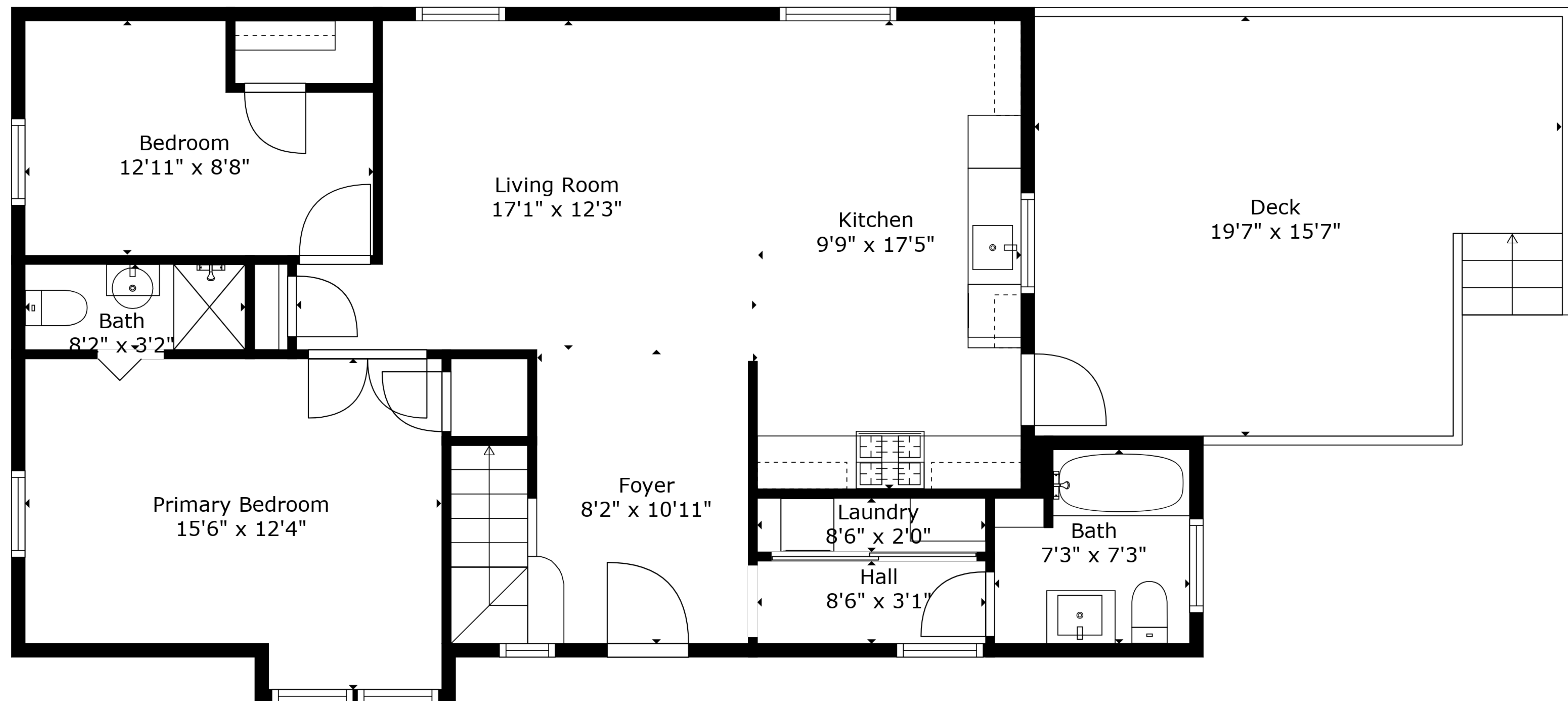
Floor 1
