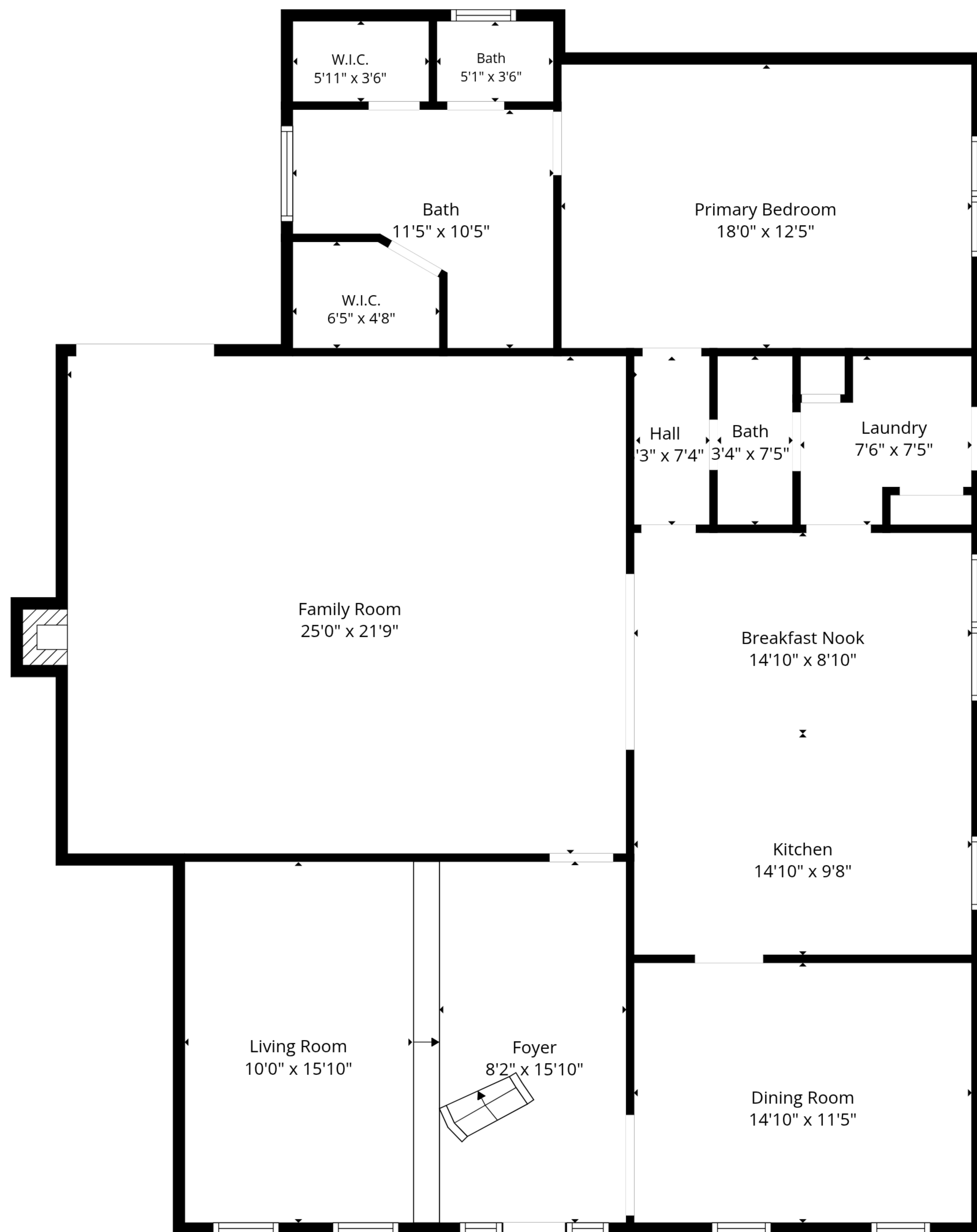
1st Floor
