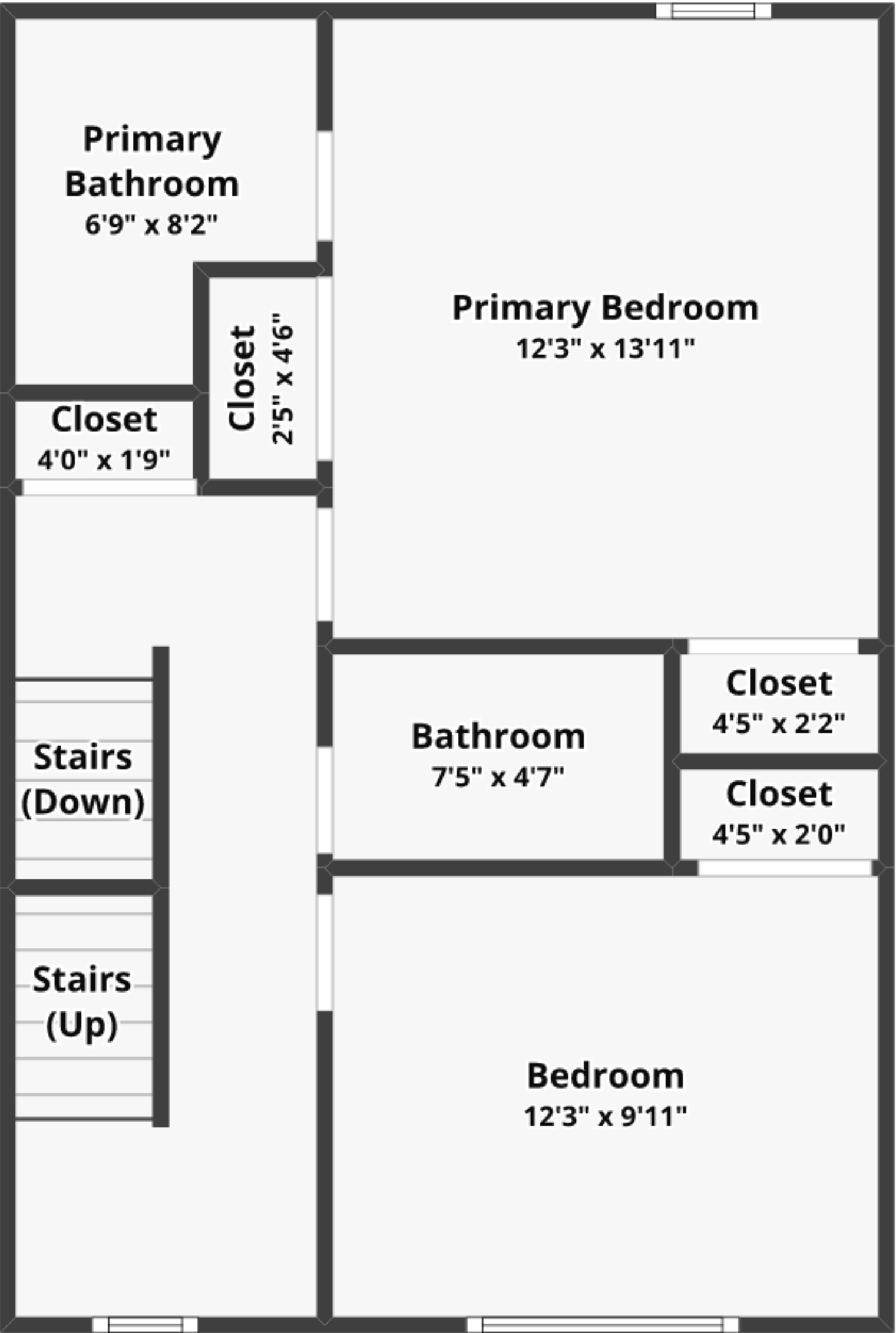
FLOOR 2 Finished area: ~511.53 sq. ft. Unfinished area: ~0.00 sq. ft.
