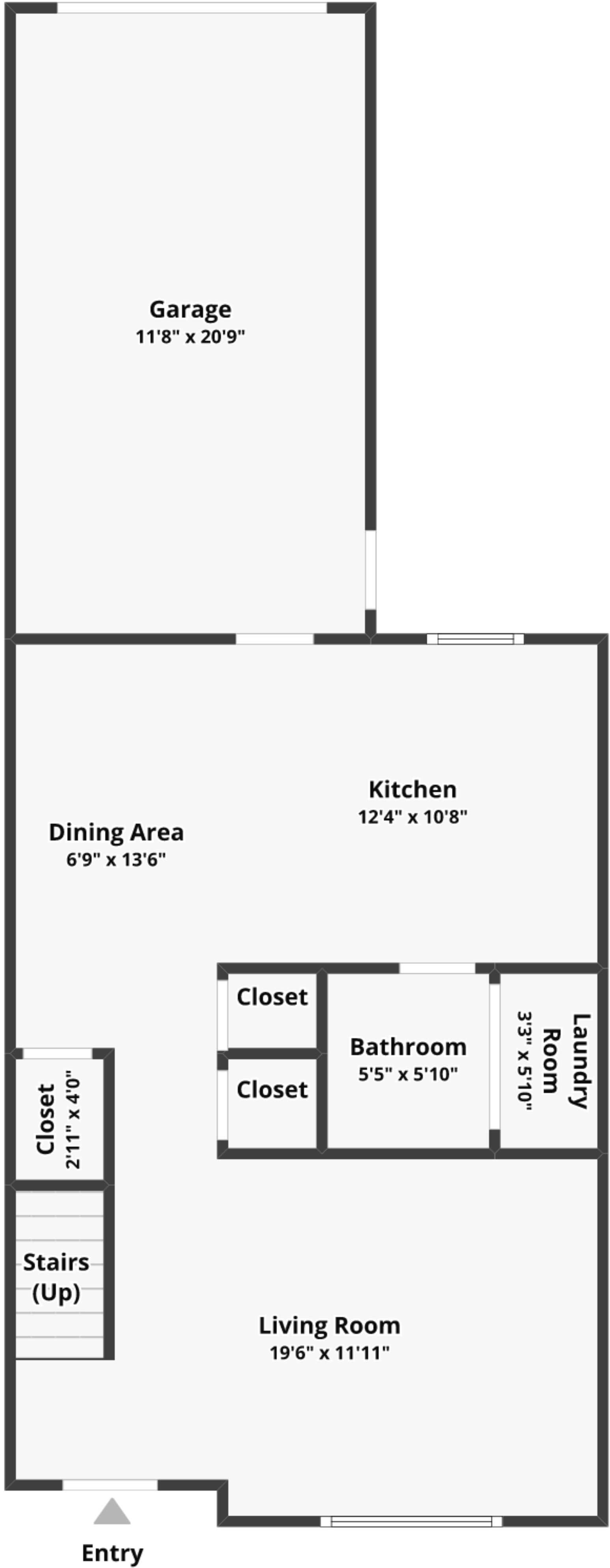
FLOOR 1 Finished area: ~519.78 sq. ft. Unfinished area: ~0.00 sq. ft.
