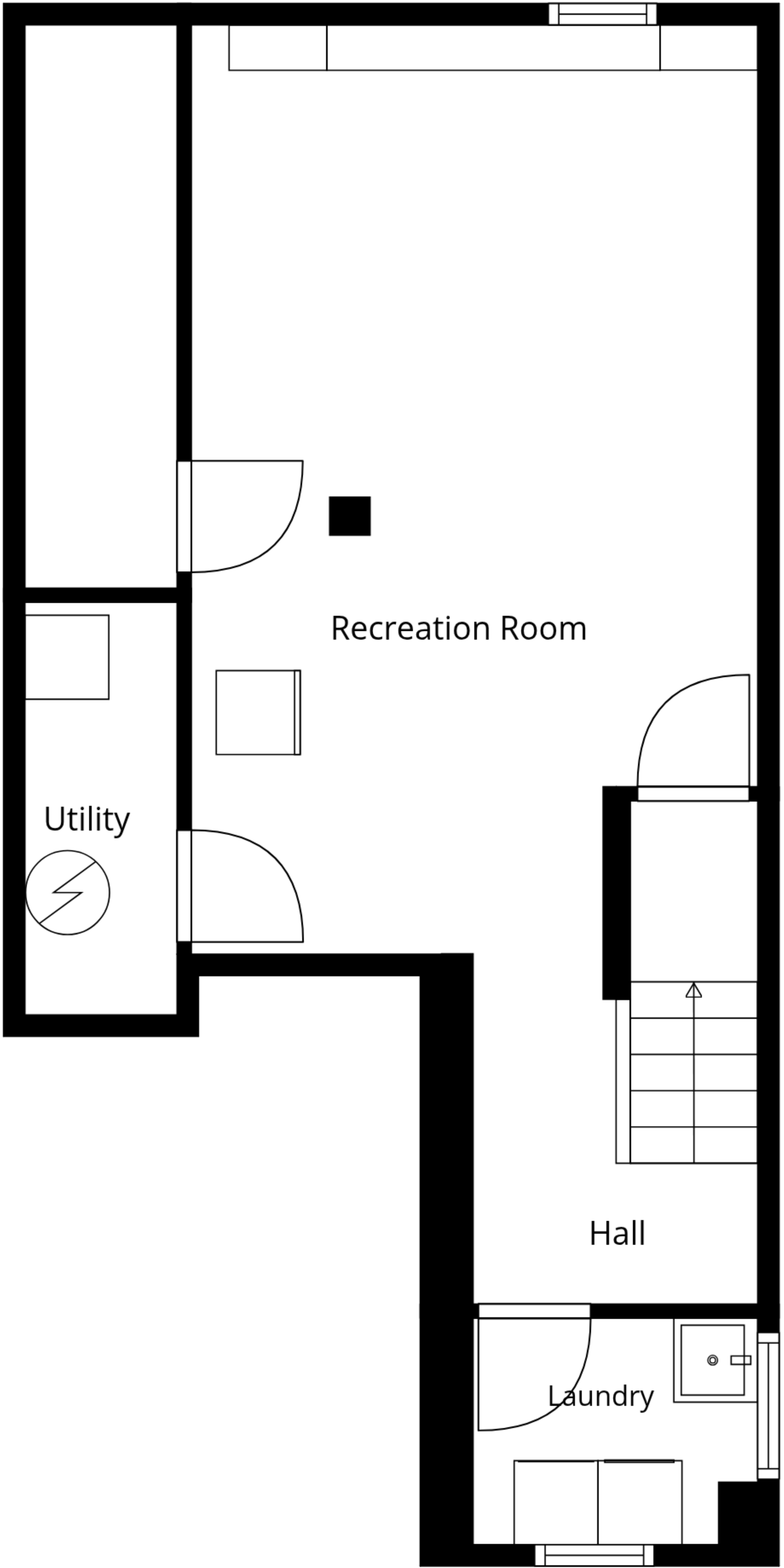
Basement
