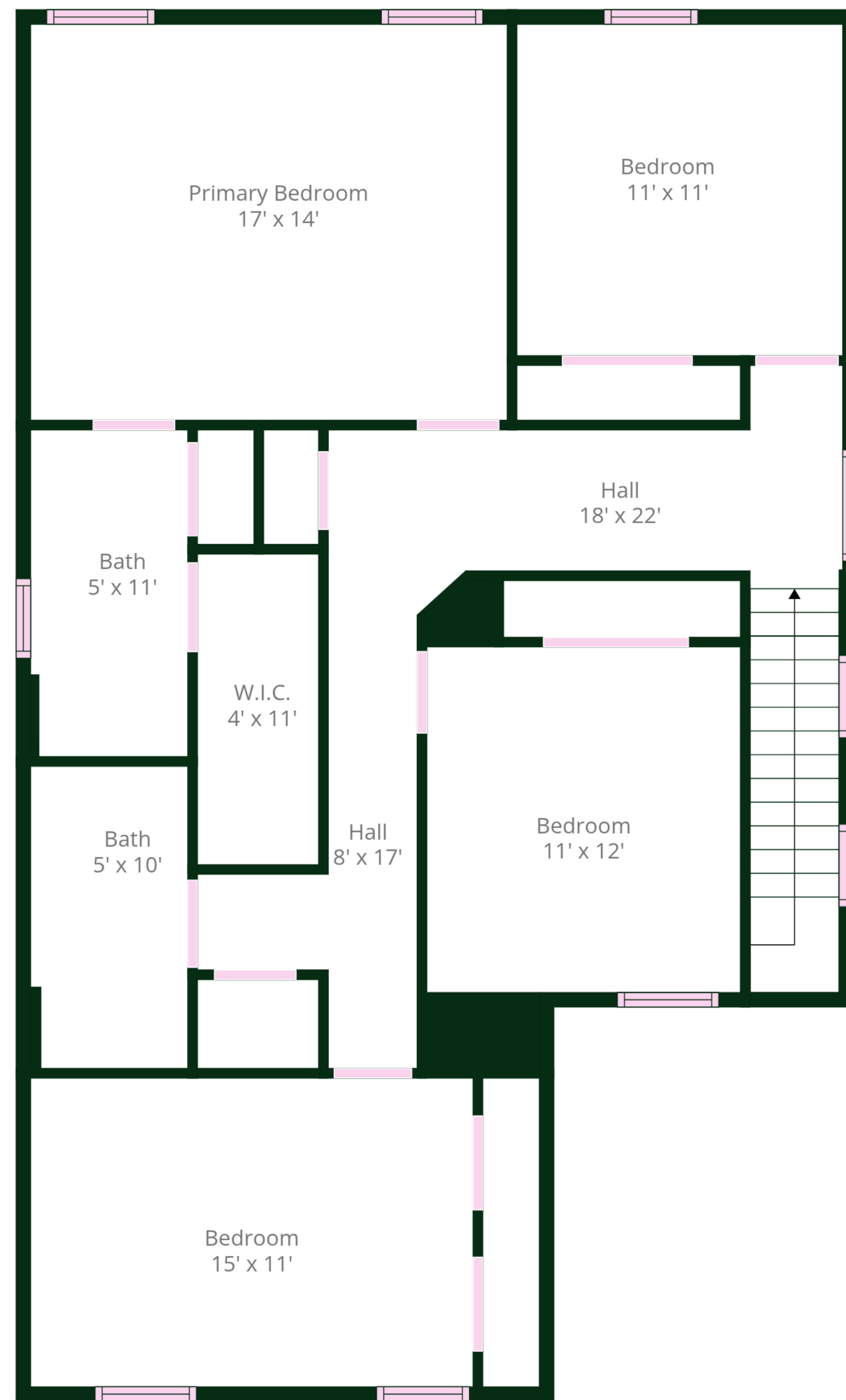
2nd Floor
