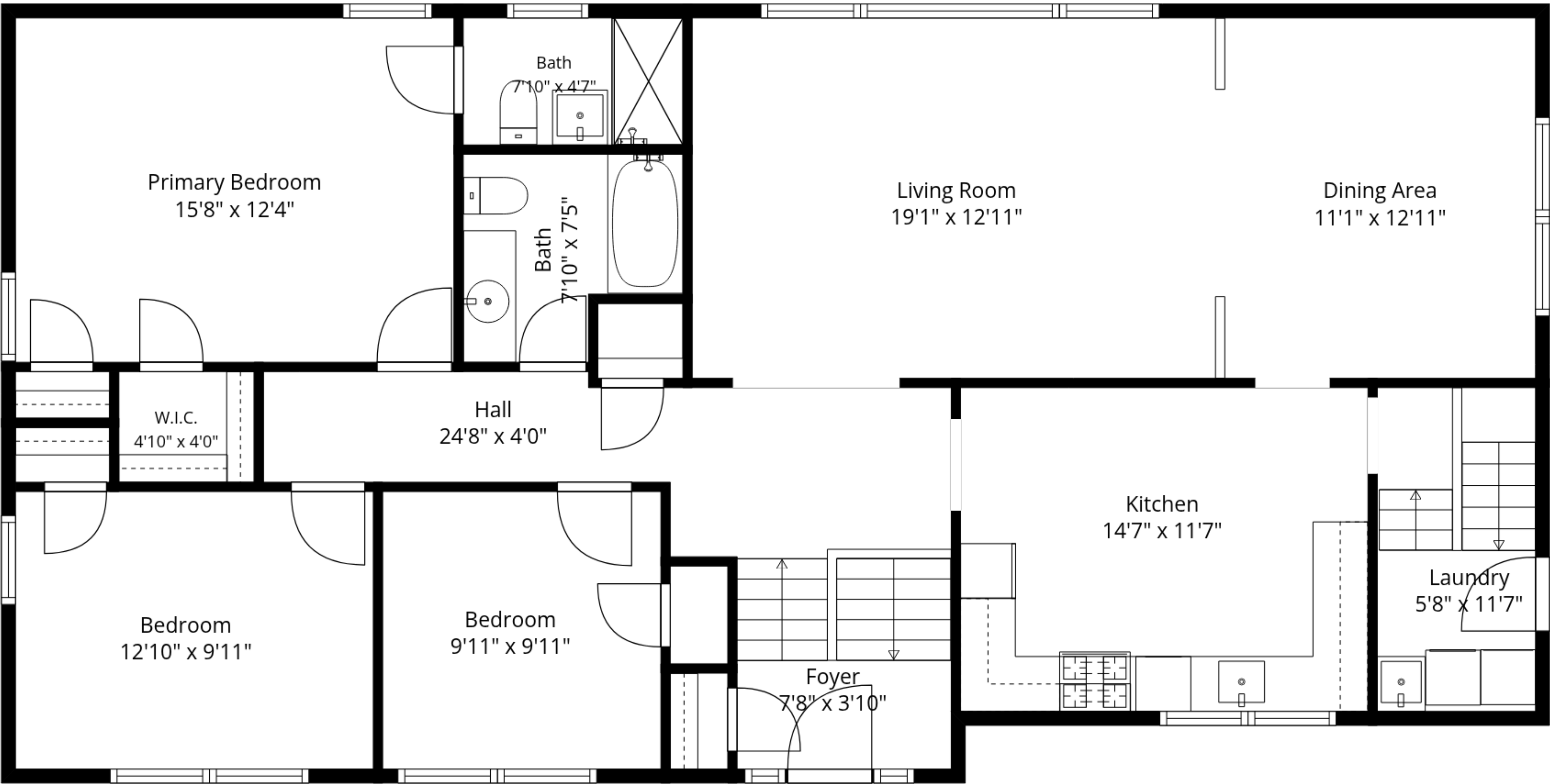
2nd Floor
