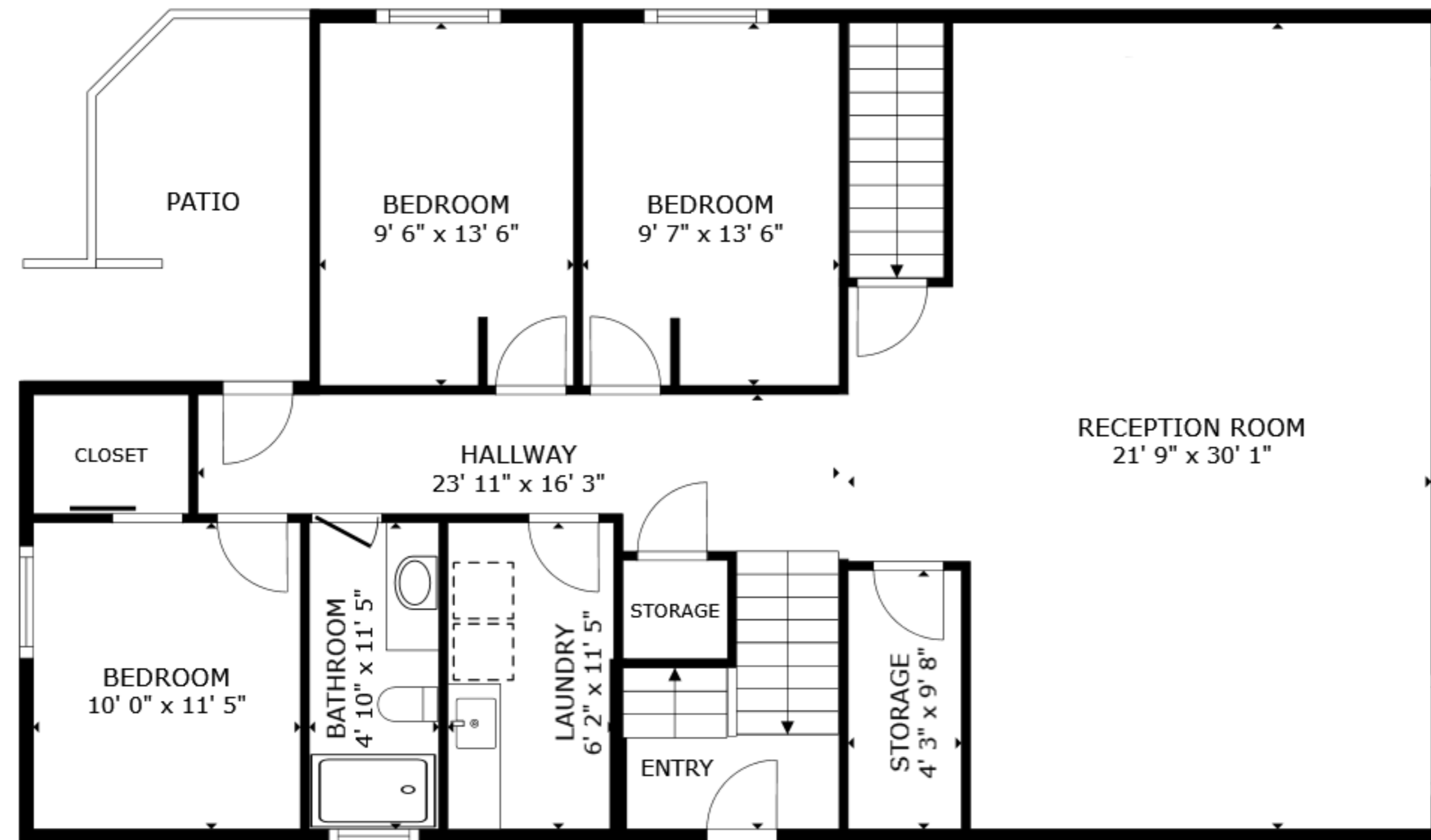
FLOOR 2
