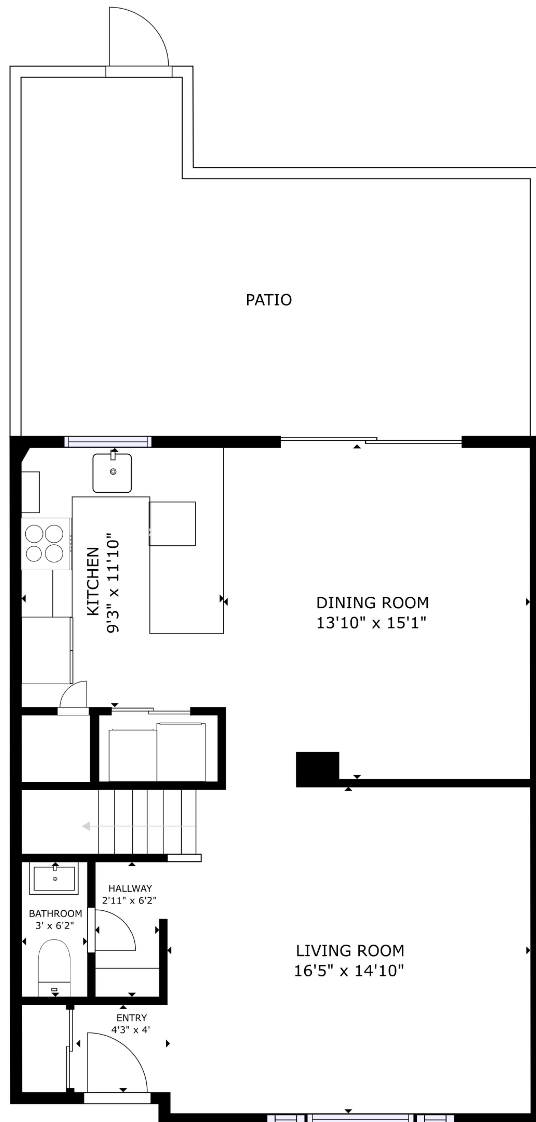
FLOOR 1
