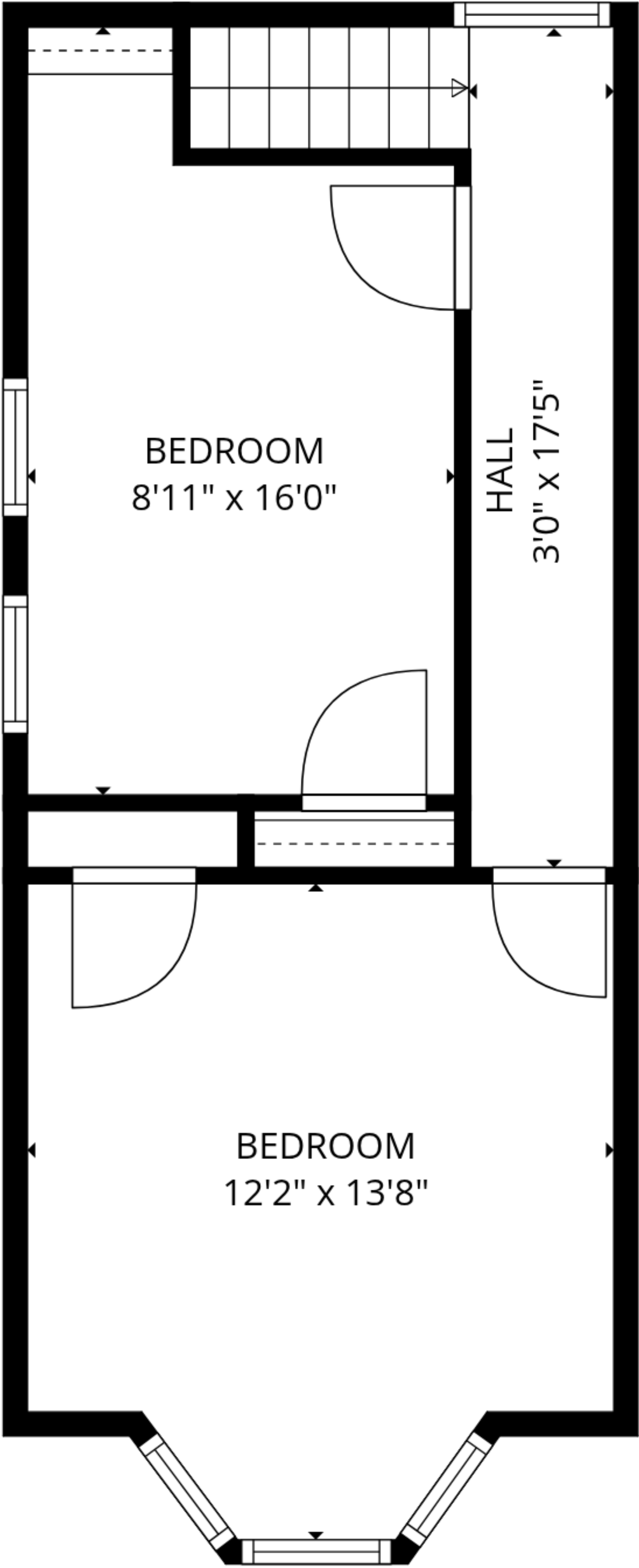
3rd floor
