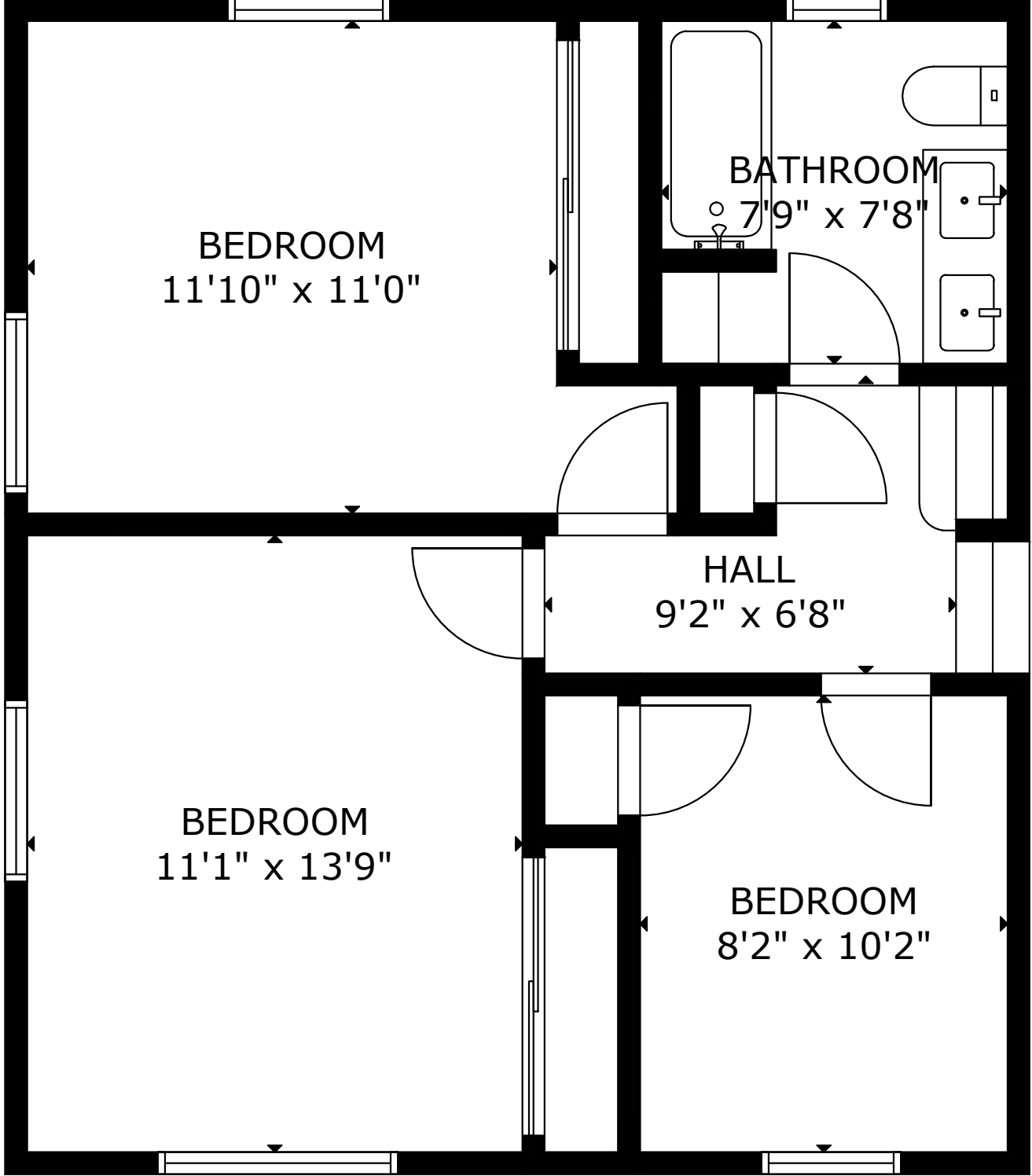
SECOND FLOOR
