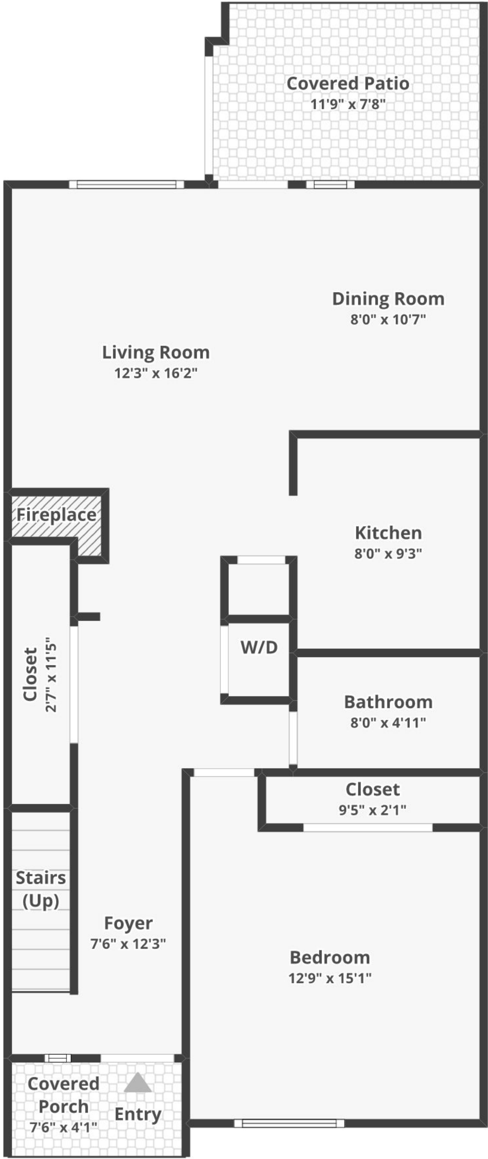
FLOOR 1
