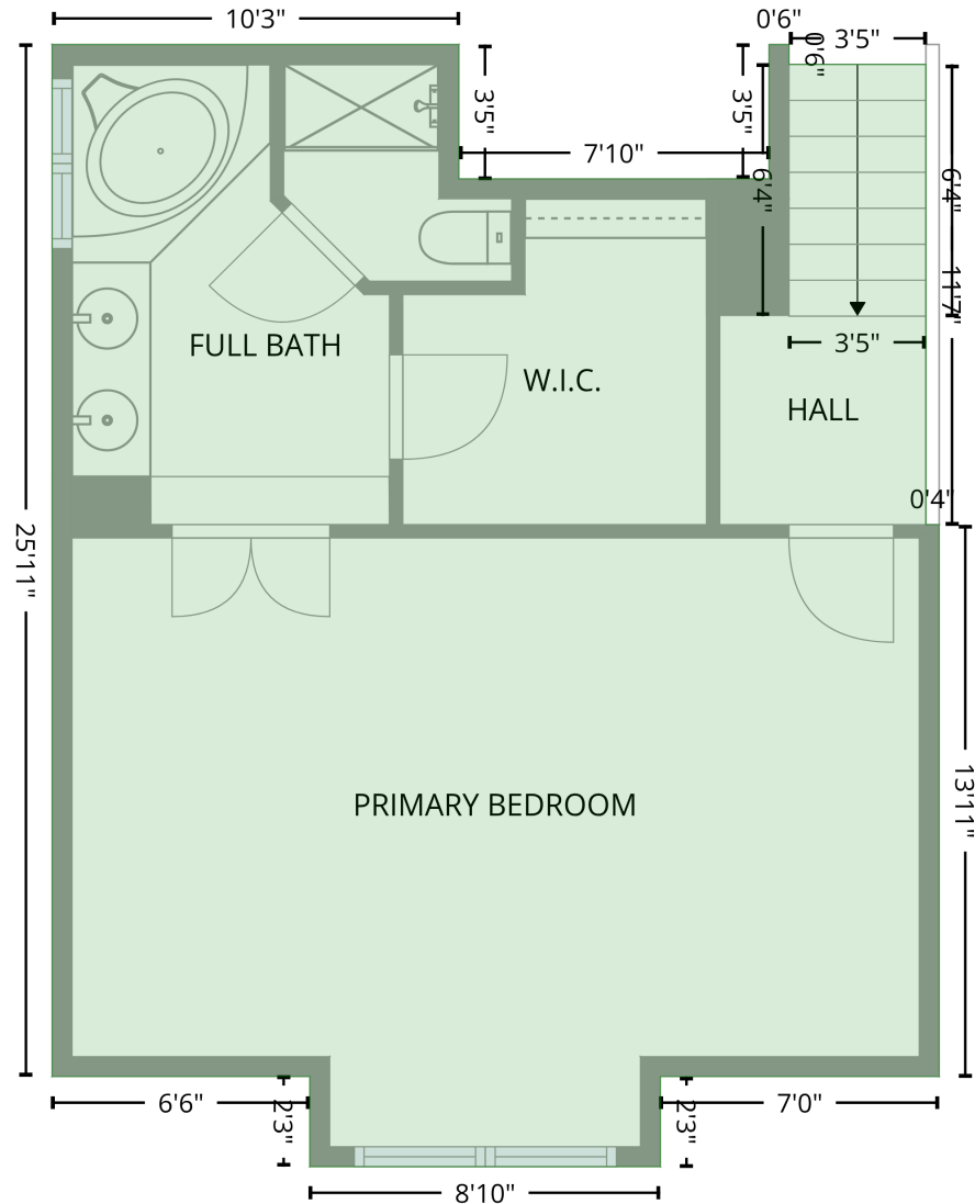
FLOOR 4 [AREA: 566]
