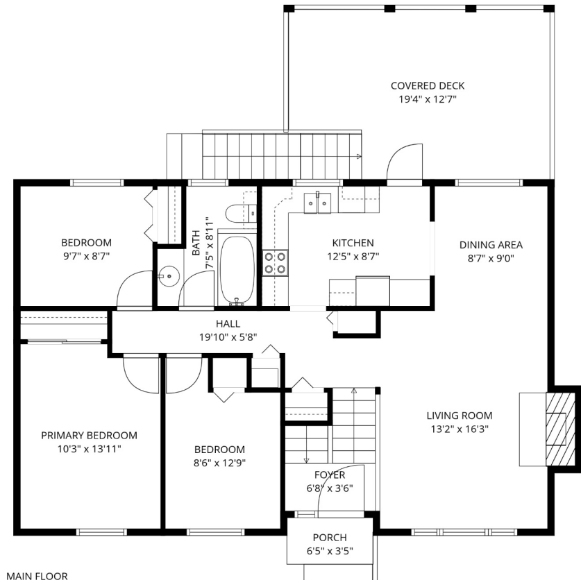
MAIN FLOOR
