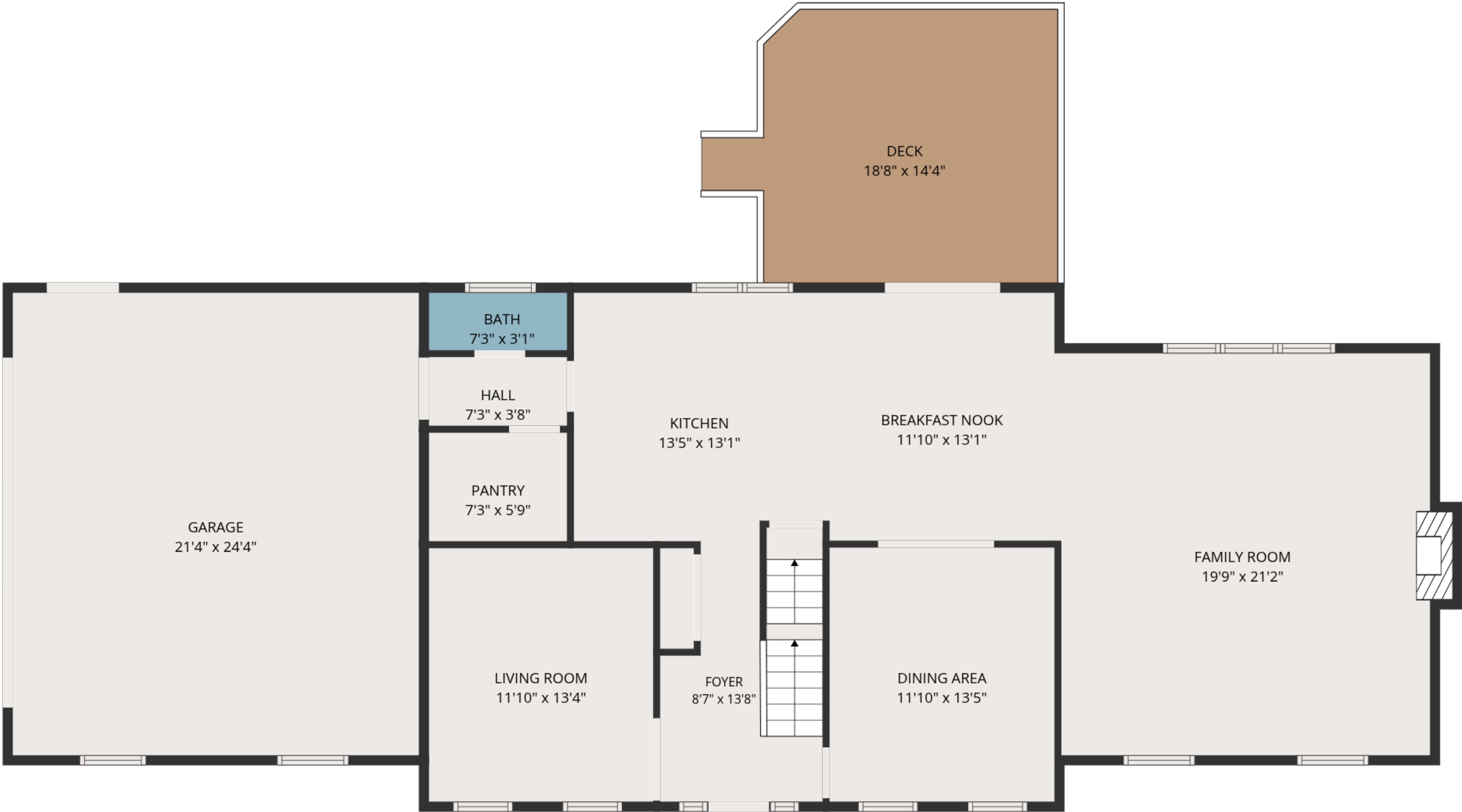
1ST FLOOR
