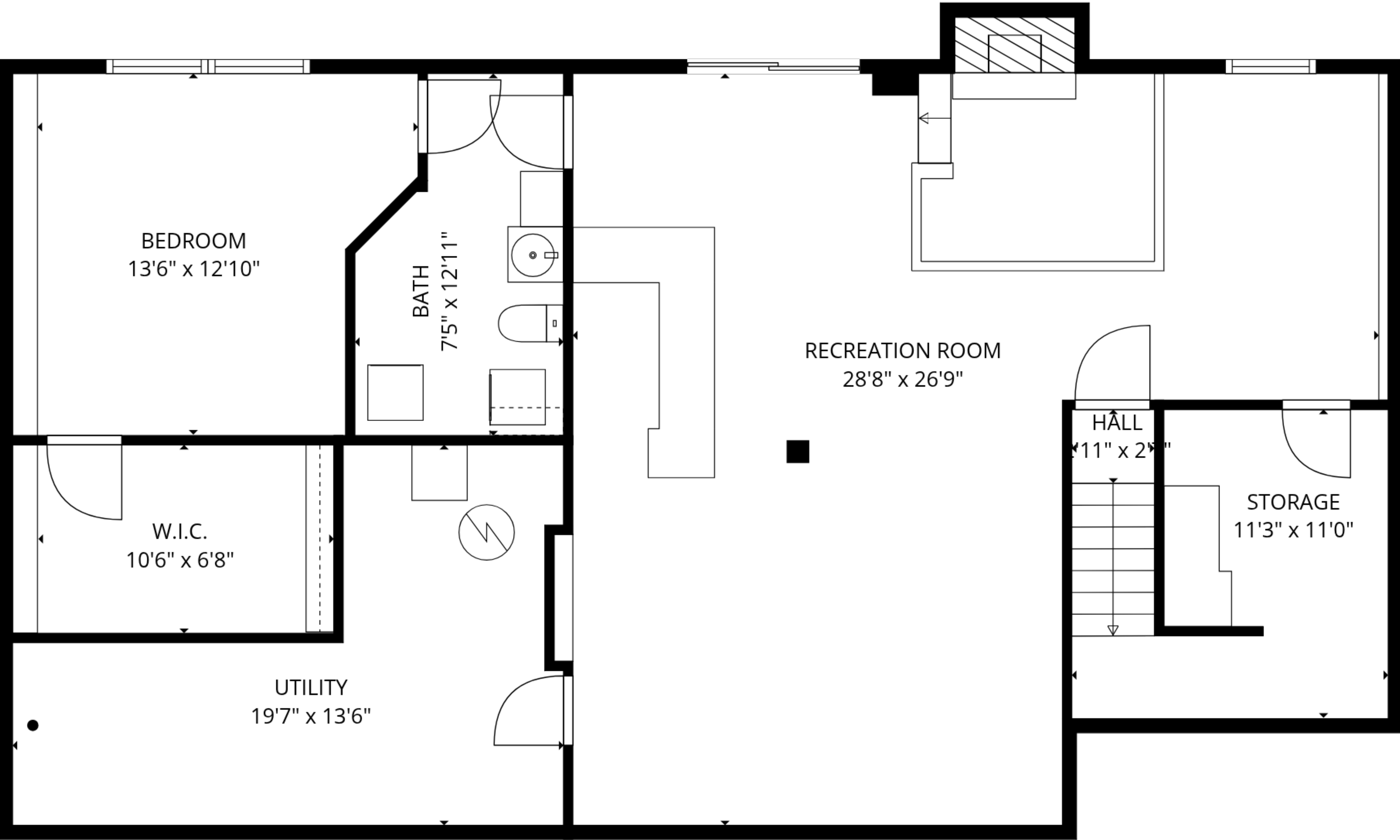
Basement 1
