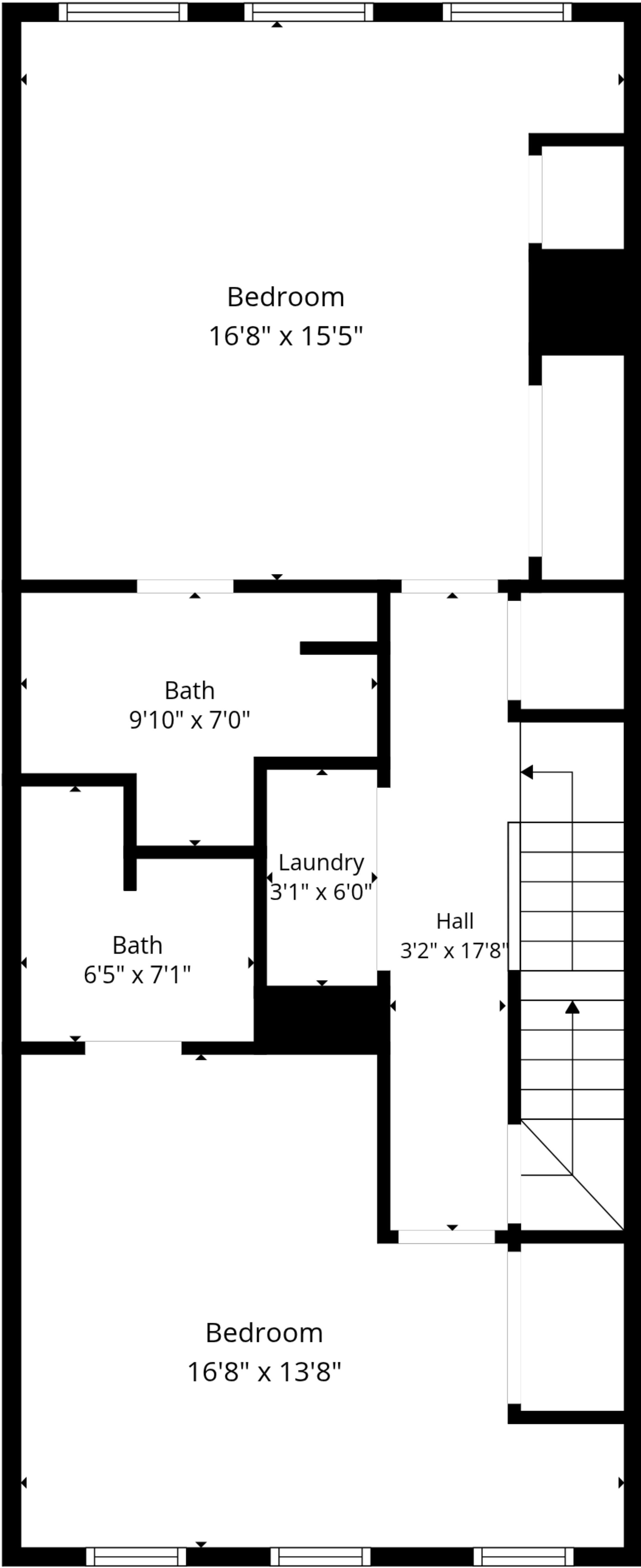
2nd Floor
