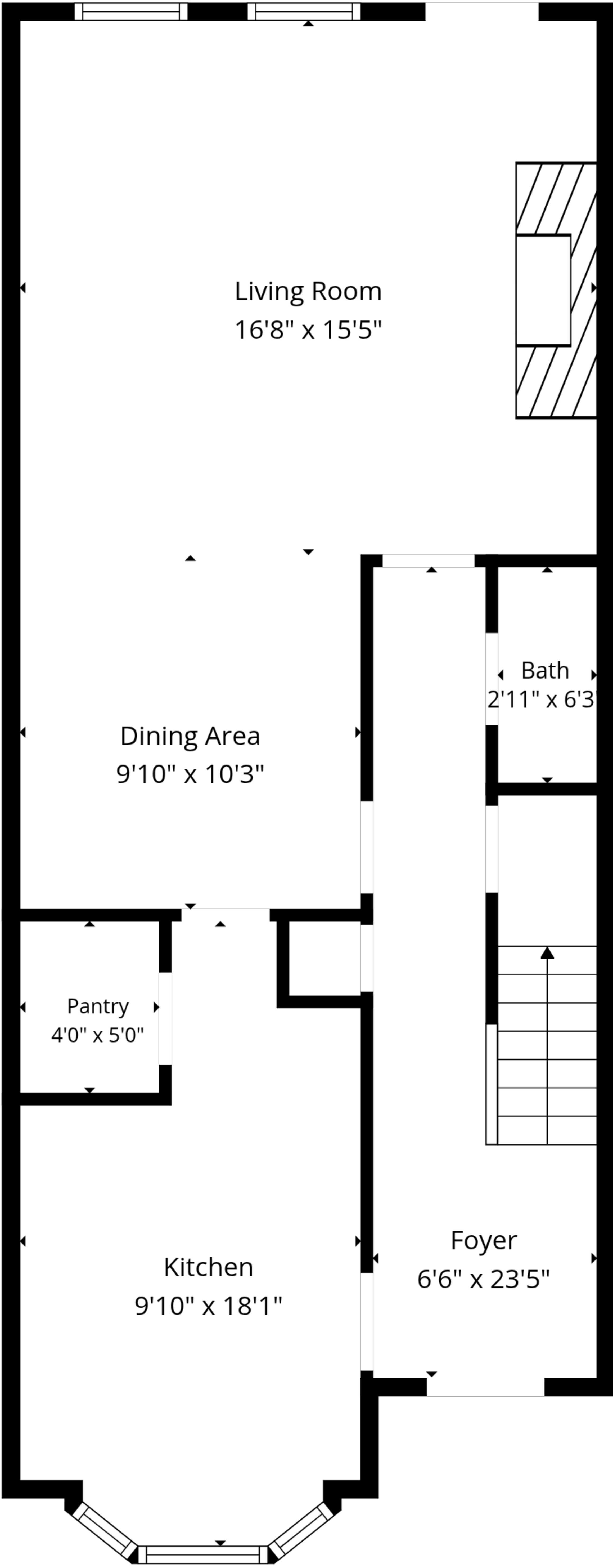
1st Floor
