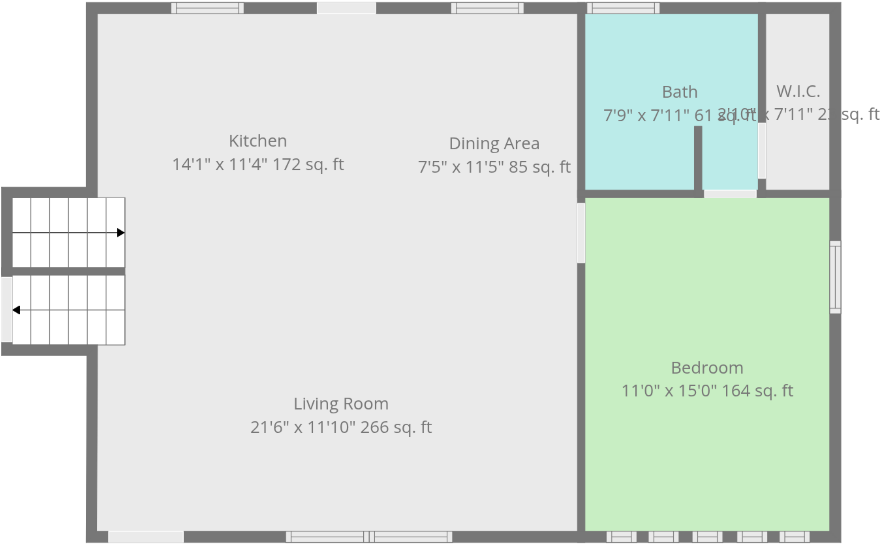
2nd Floor
