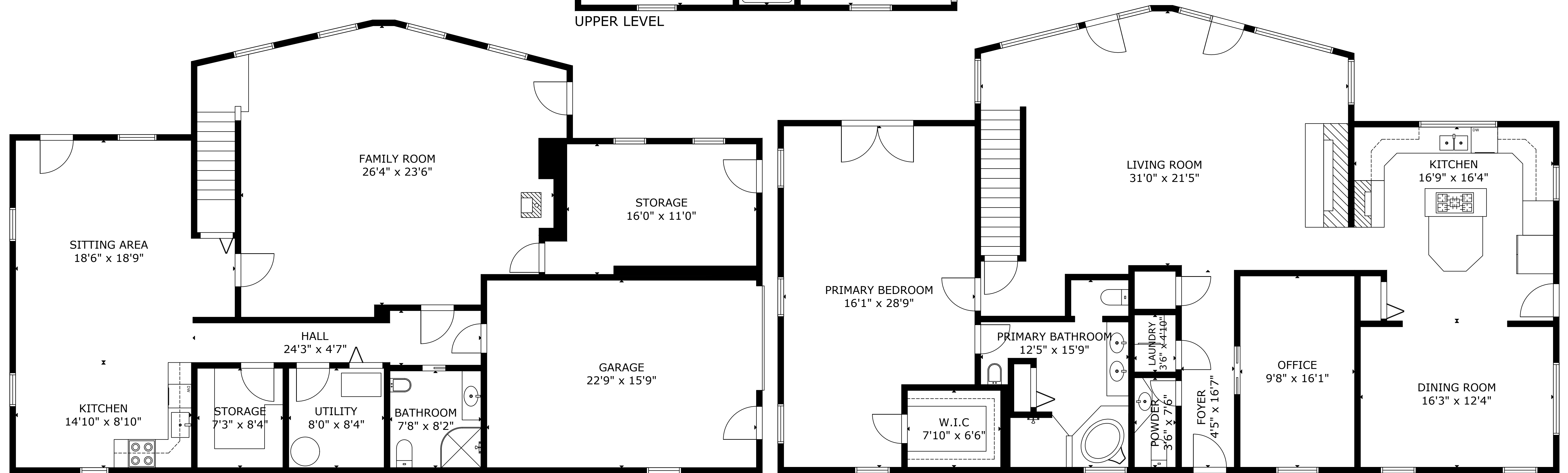
LOWER FLOOR
