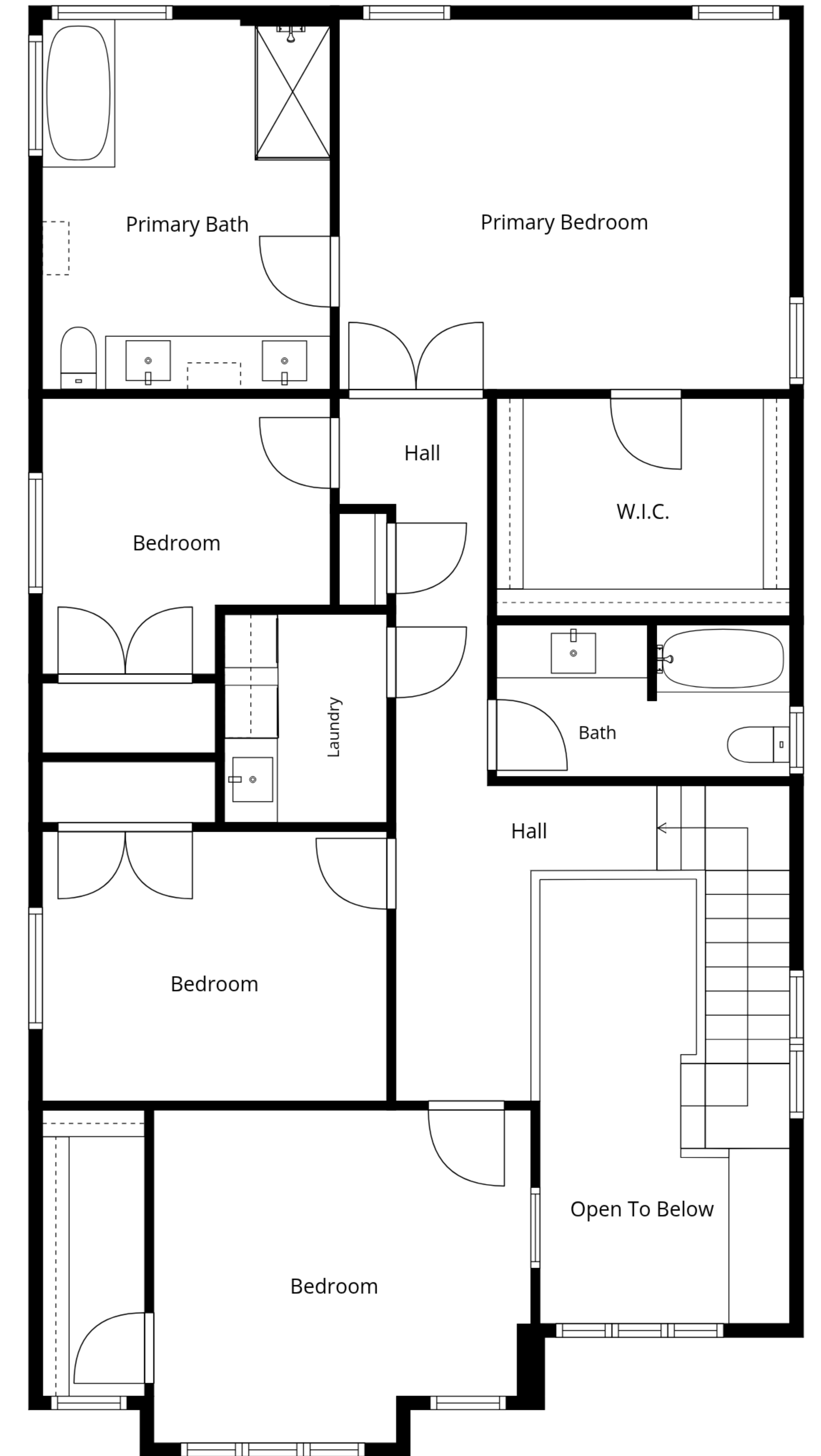
2nd Floor
