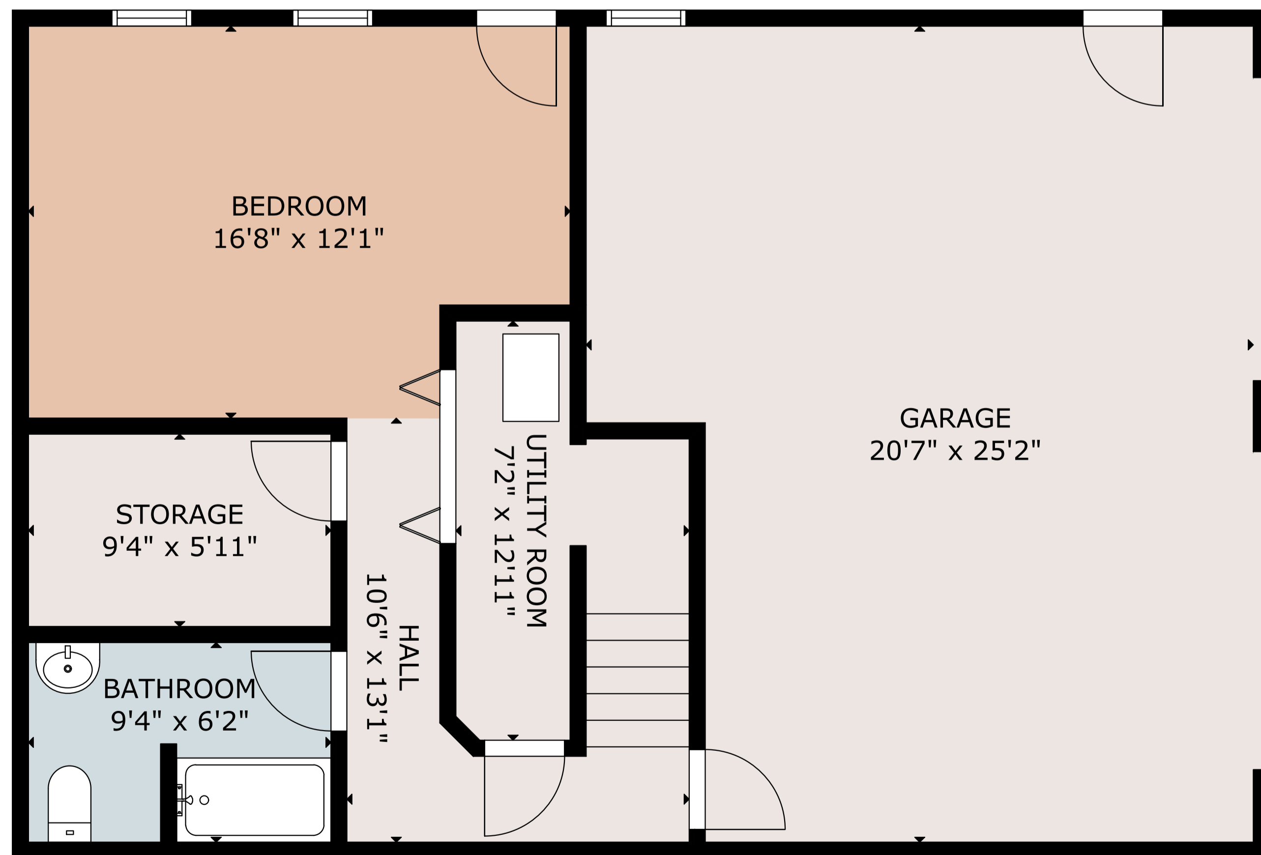
LOWER FLOOR
