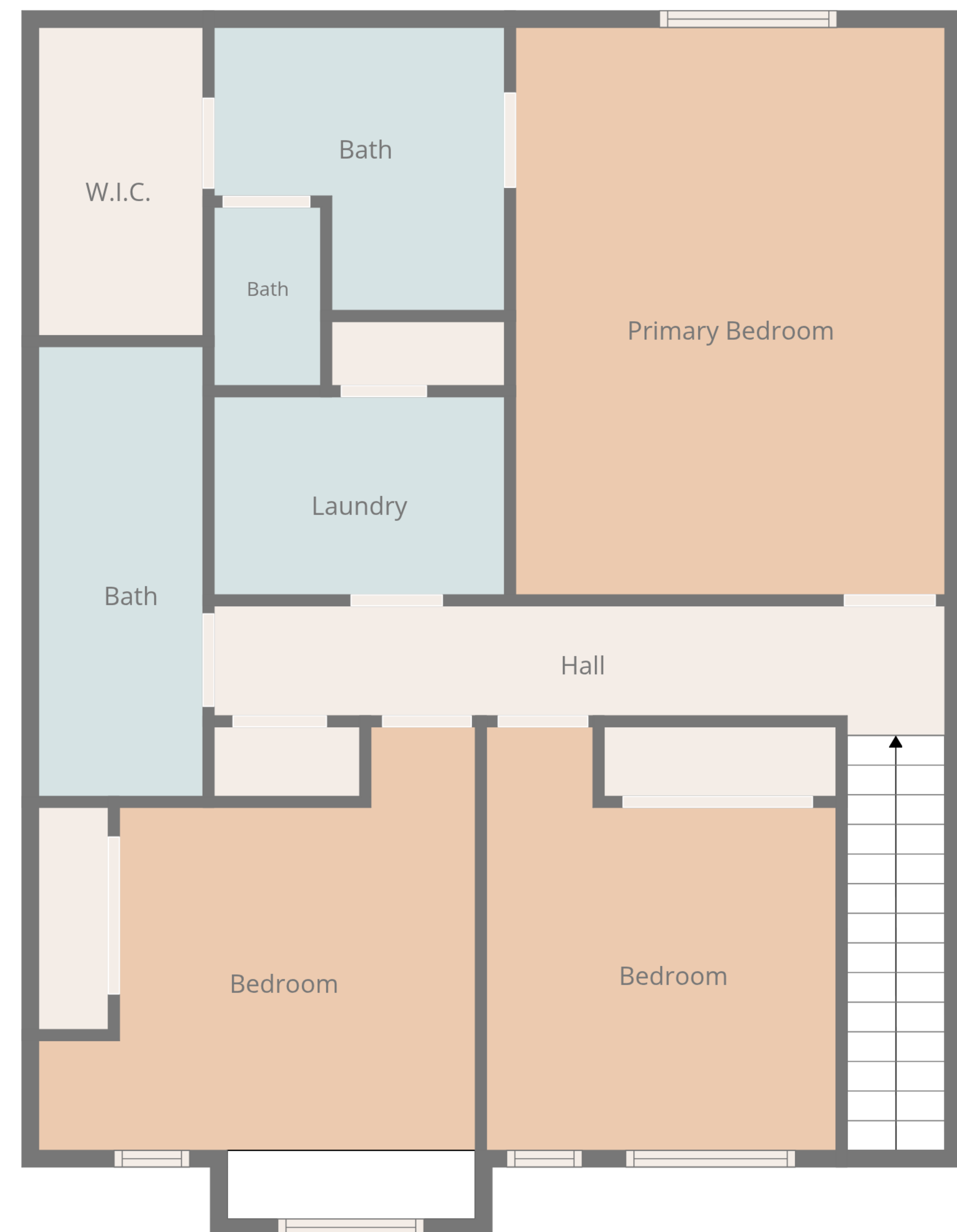
2nd Floor
