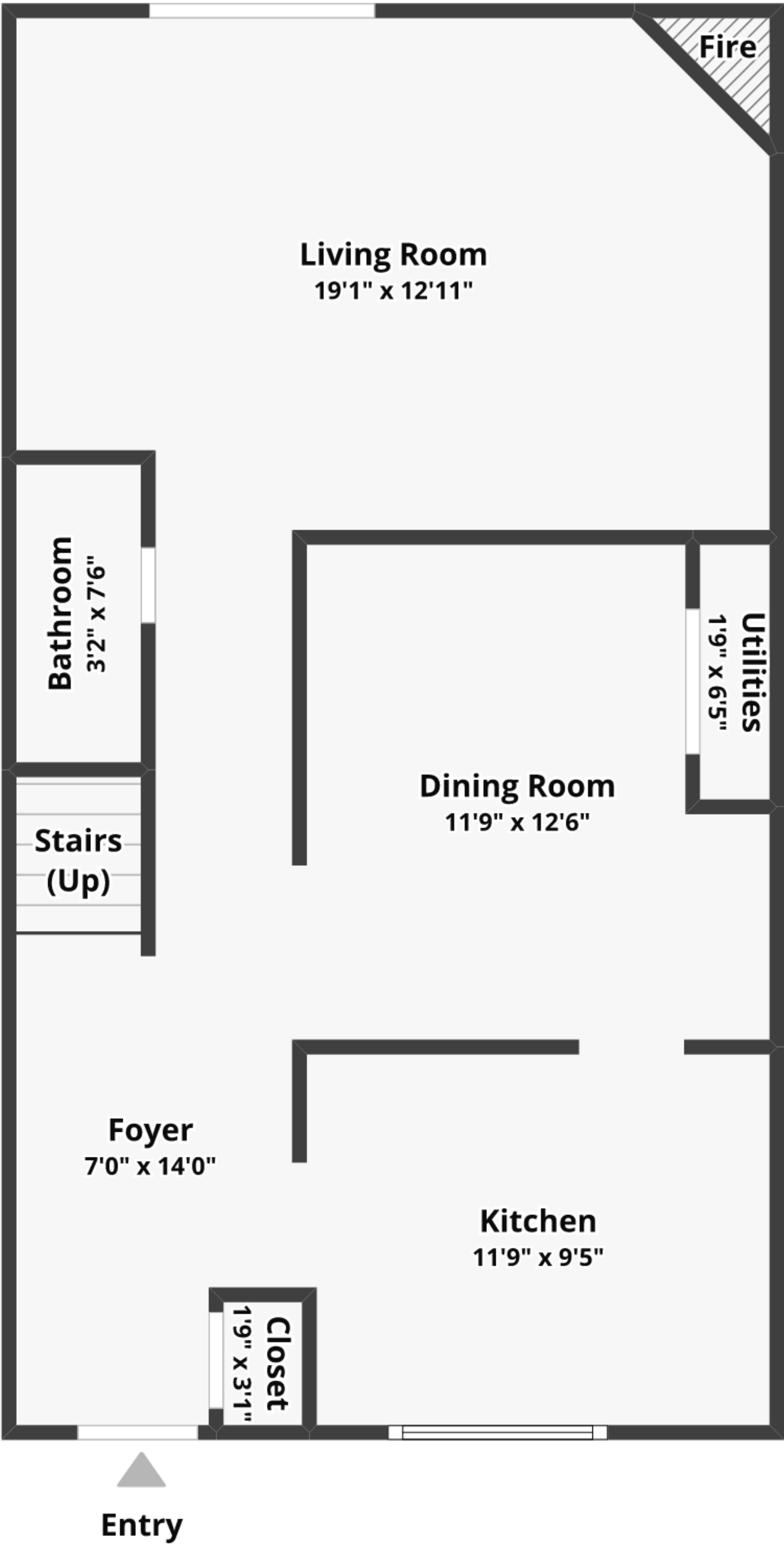
FLOOR 1 Finished area: ~637.92 sq. ft. Unfinished area: ~4.40 sq. ft.
