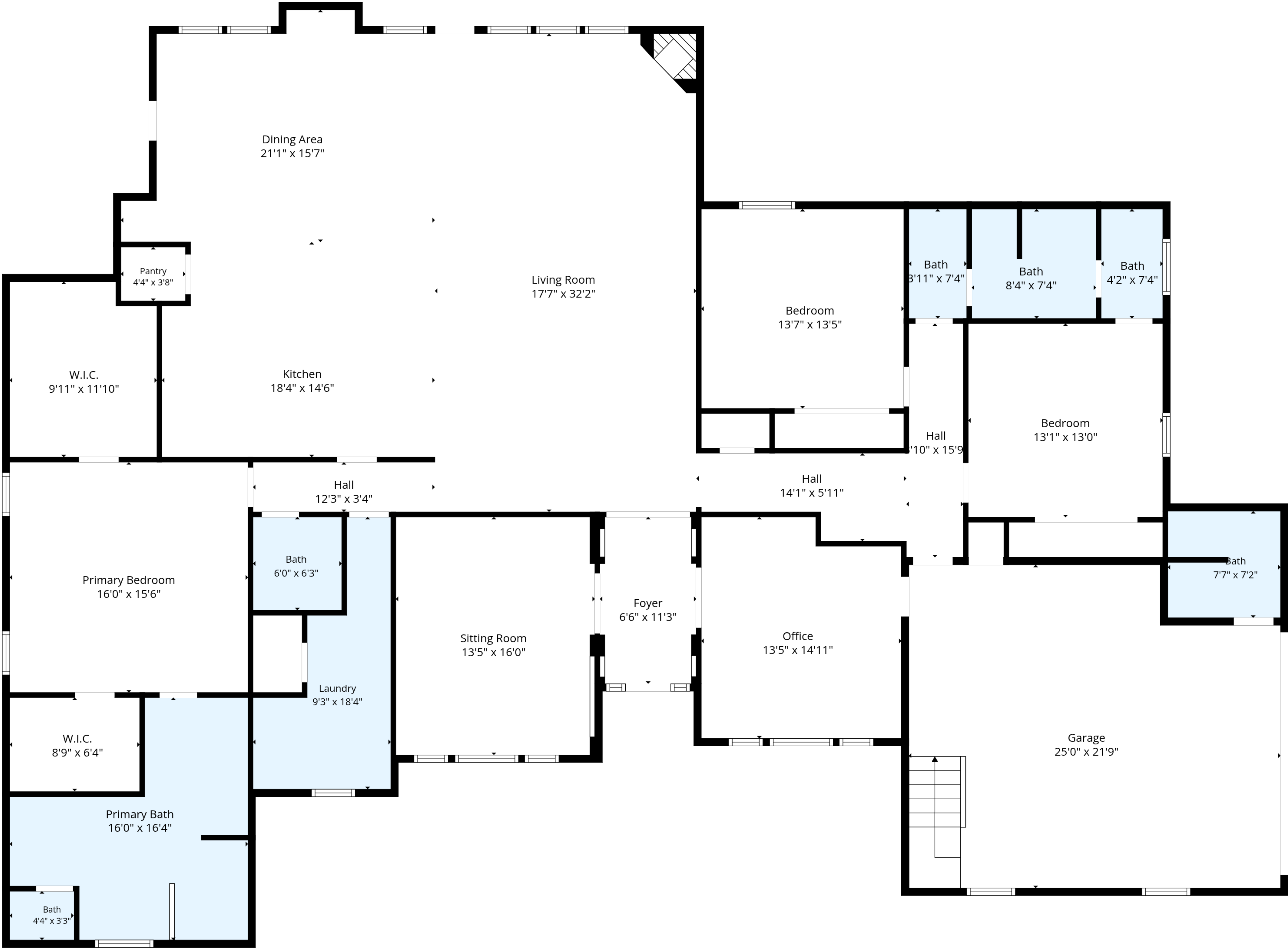
1st Floor
