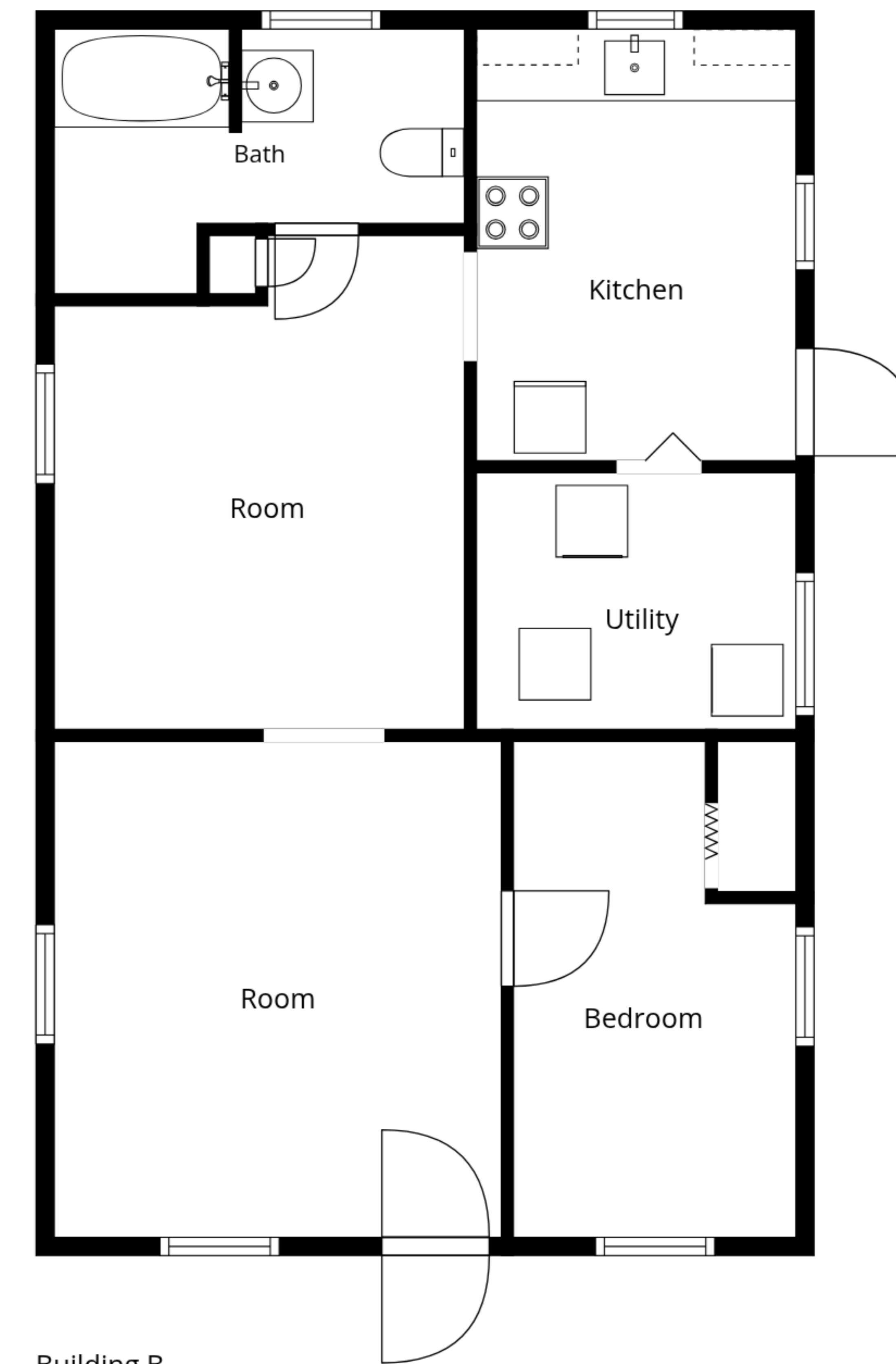
Building B
