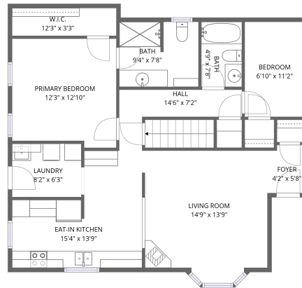
1st floor
