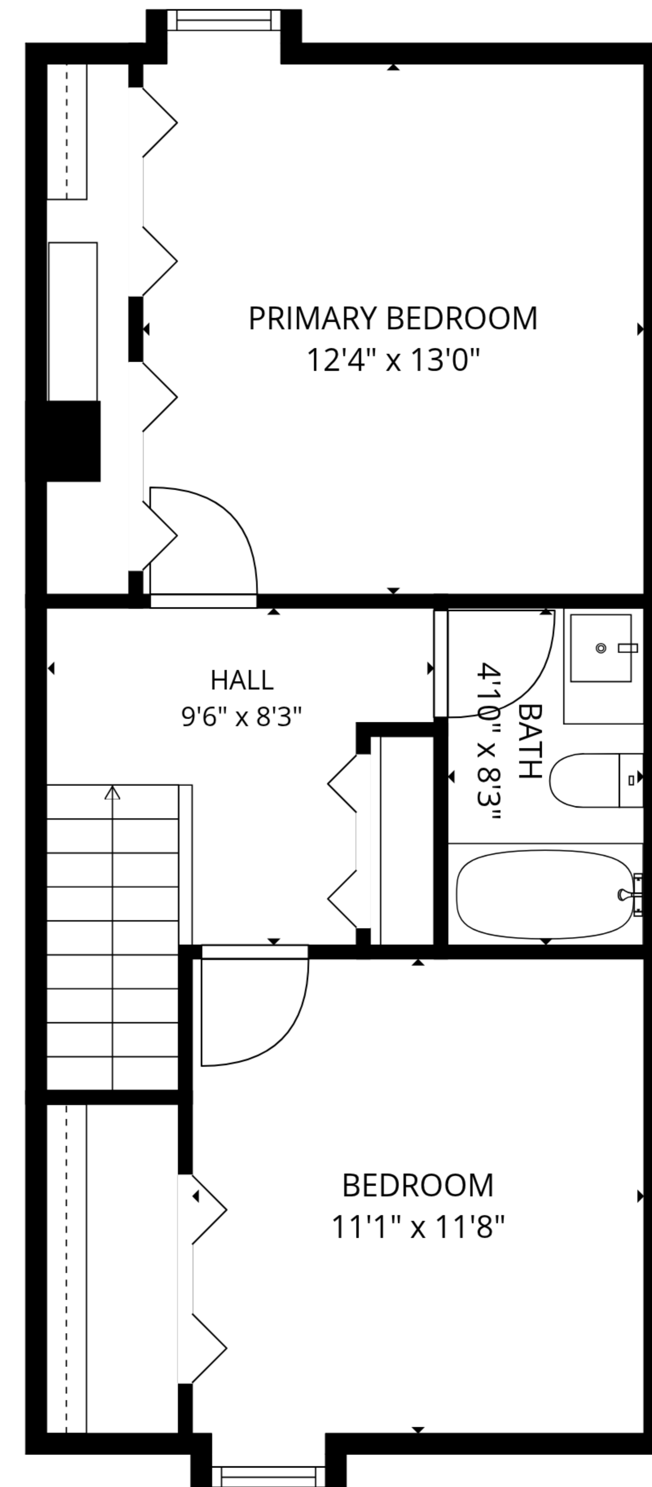
2nd floor
