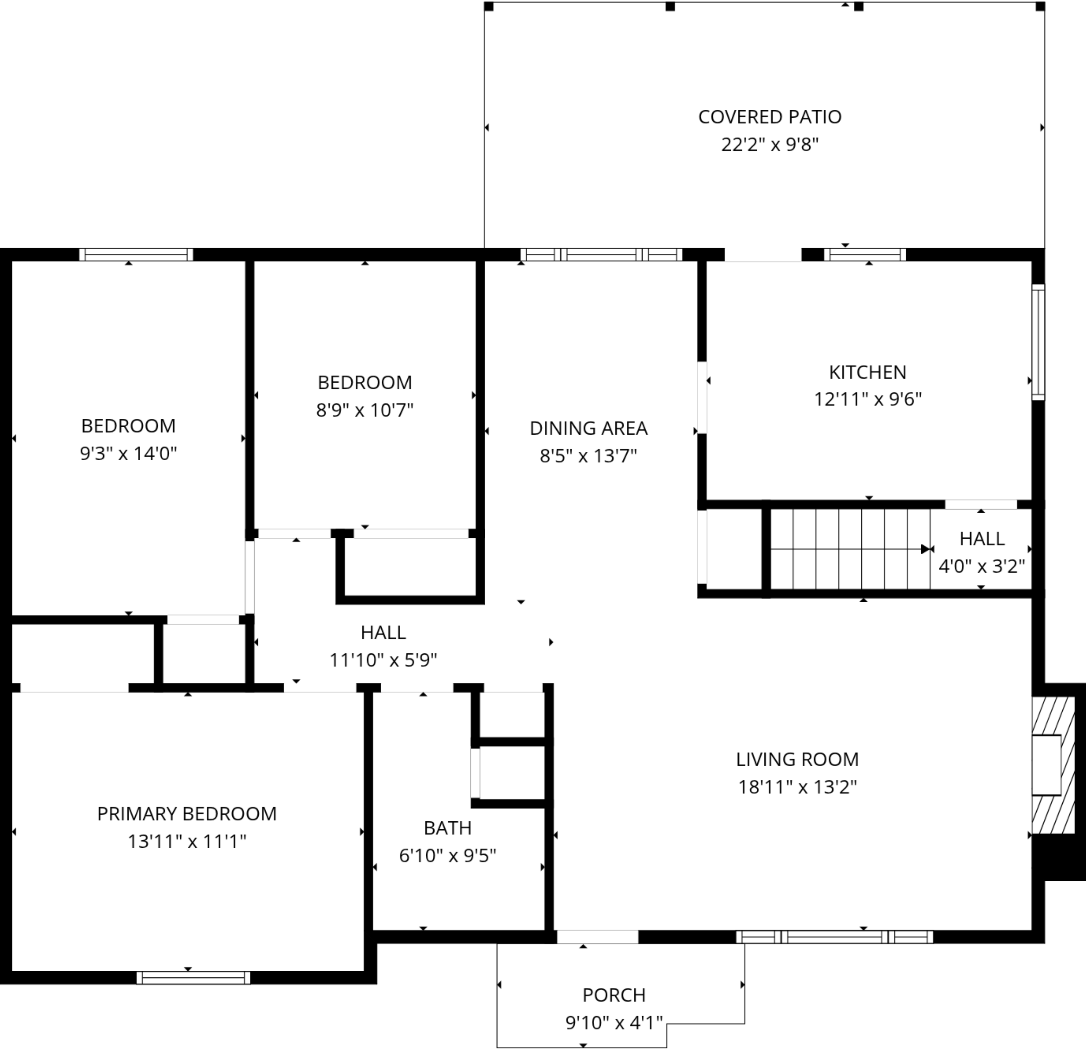
FLOOR 2
