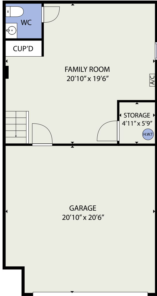
FLOOR 1
