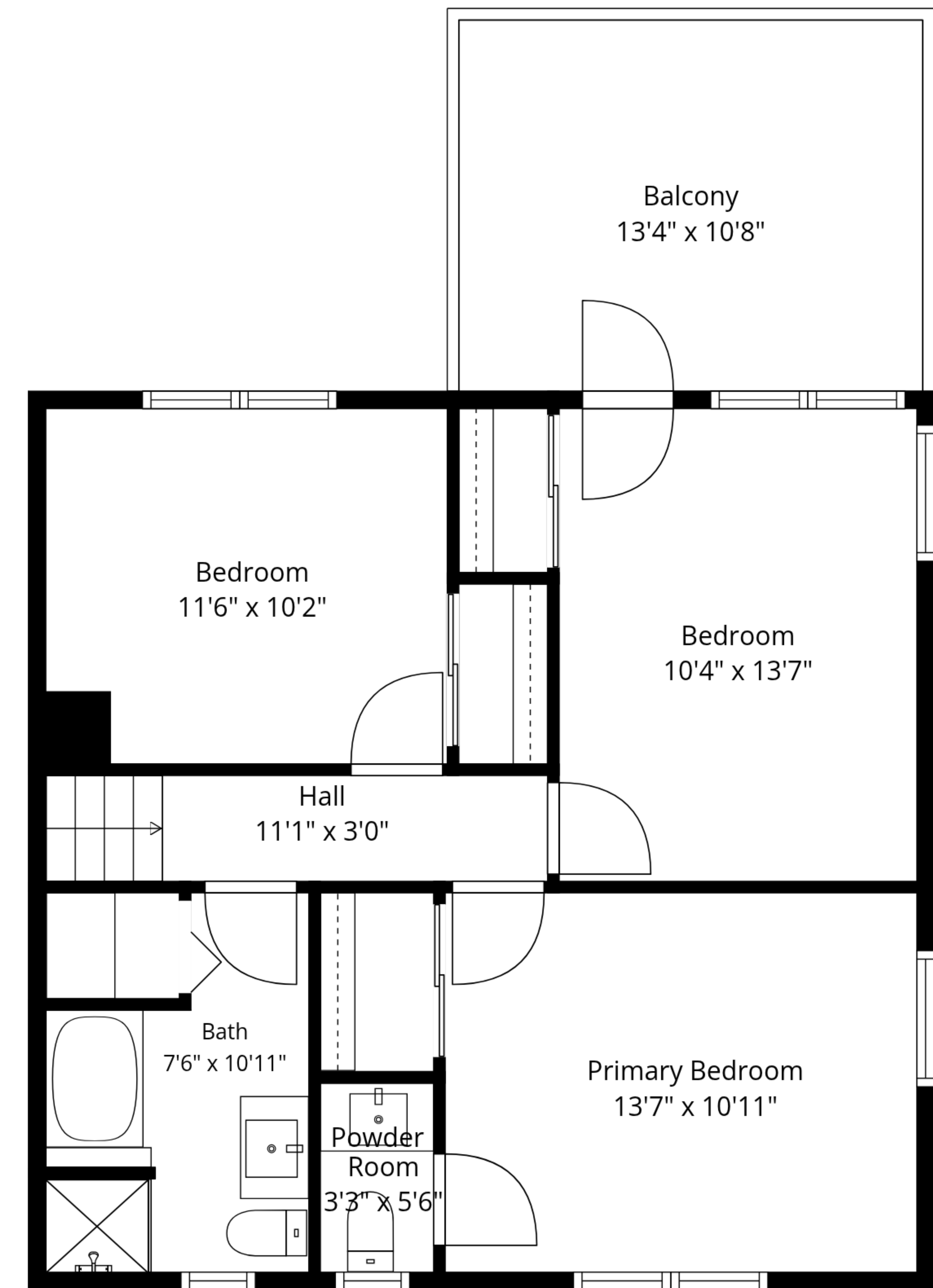
3rd Floor
