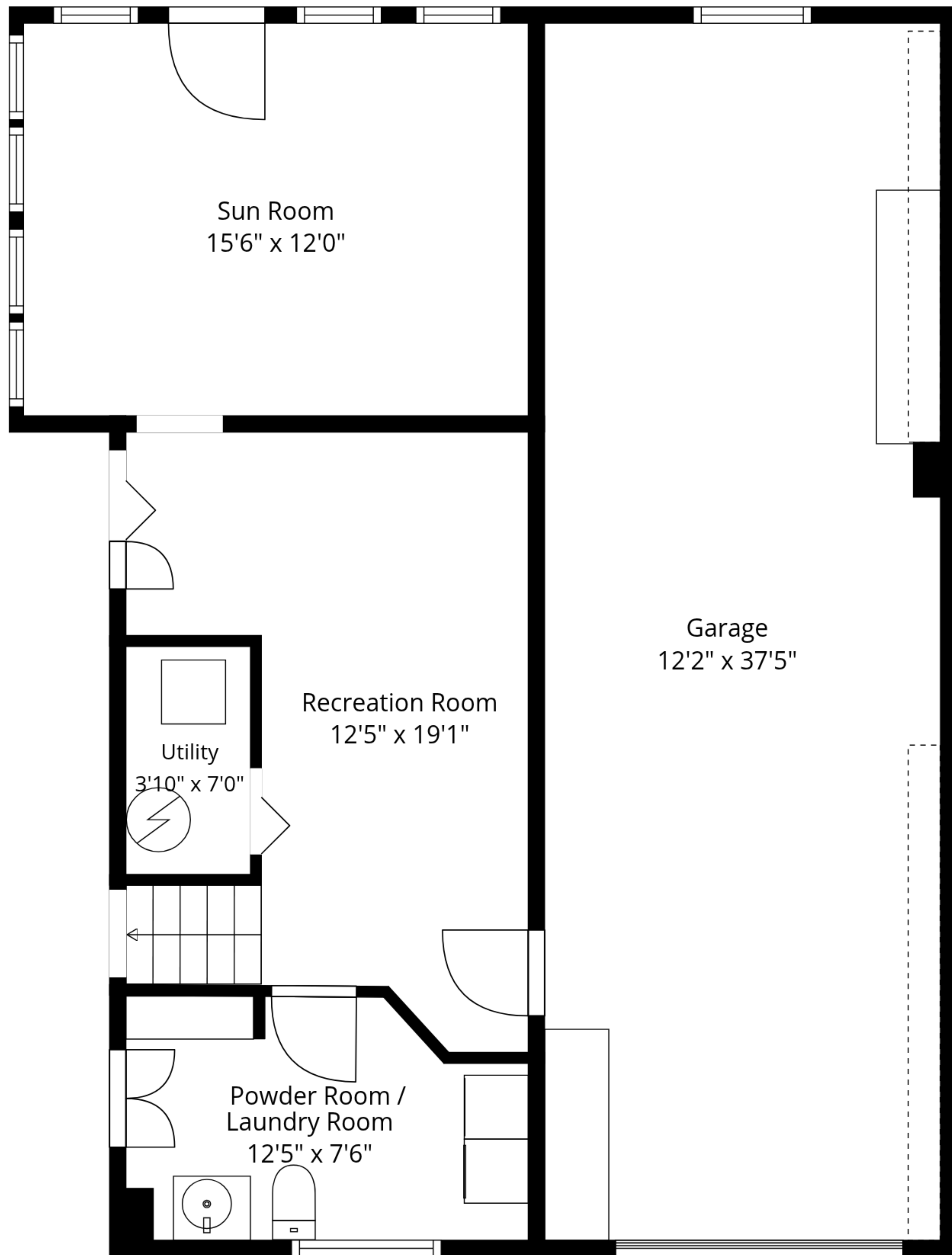
1st Floor
