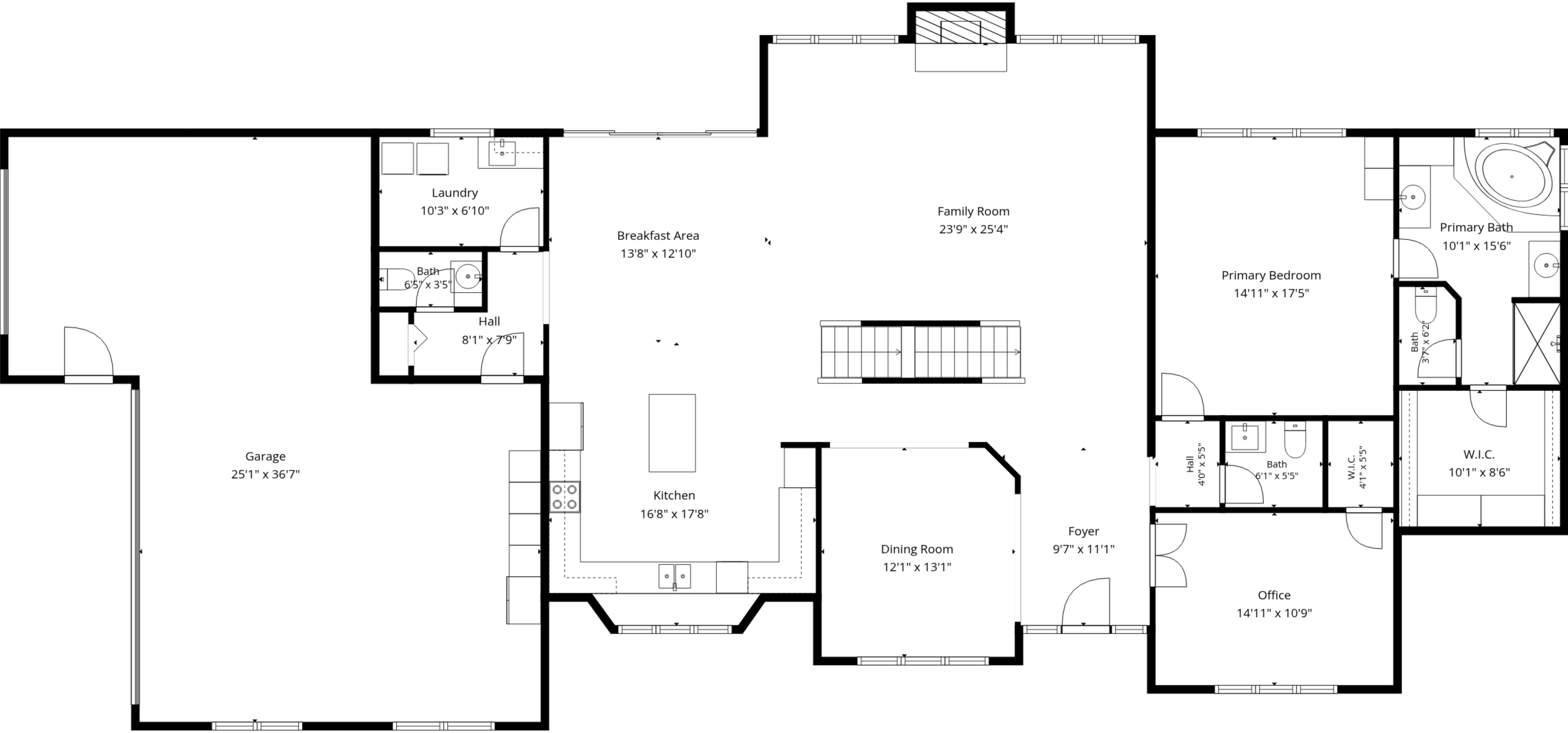
1st Floor
