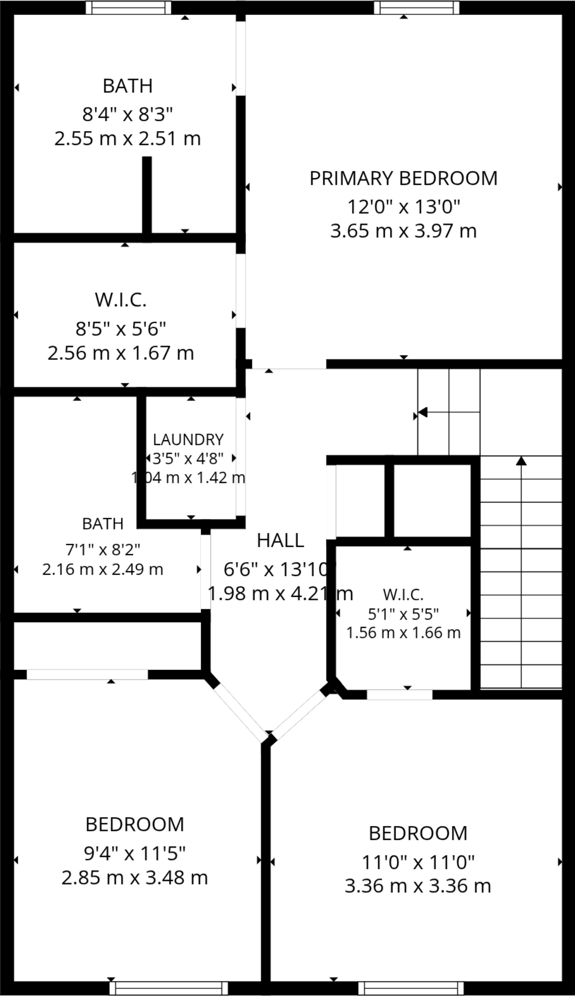
2nd floor
