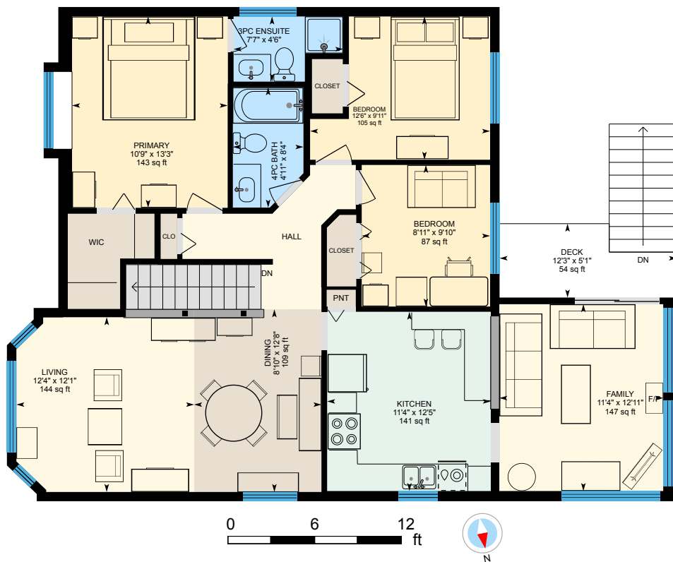
Main Floor (8ft) Exterior Area 1257.60 sq ft
