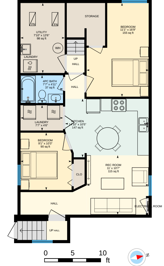
Basement (Below Grade) Exterior Area 970.39 sq ft
