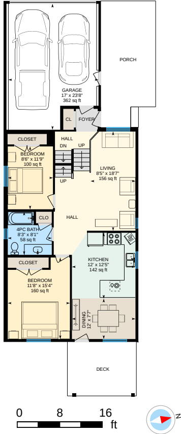
Main Floor Exterior Area 1033.25 sq ft
