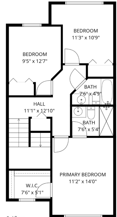
3rd floor
