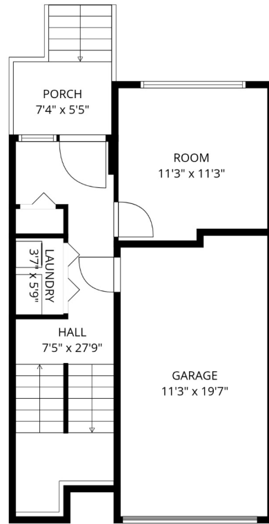
1st floor
