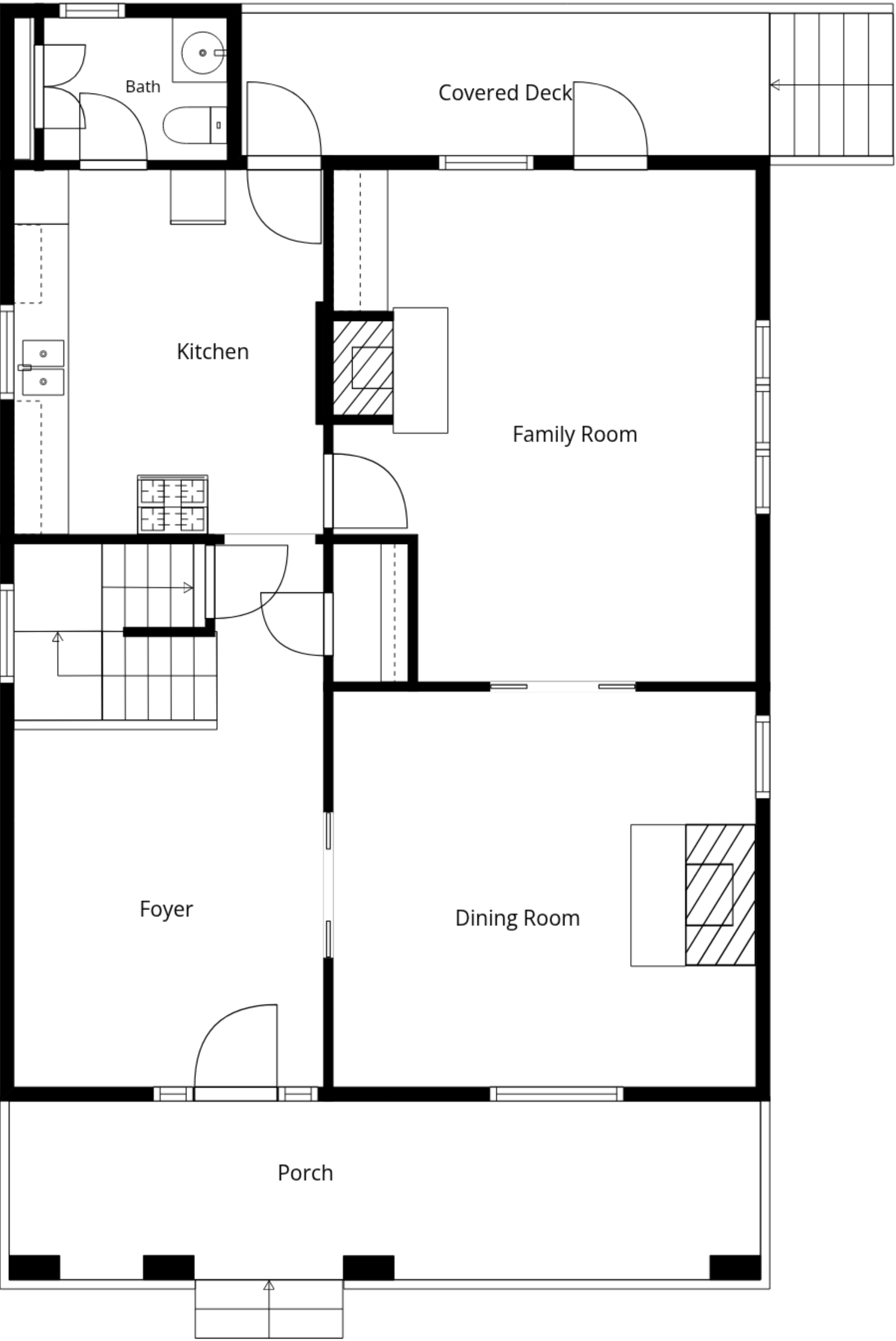
1st Floor
