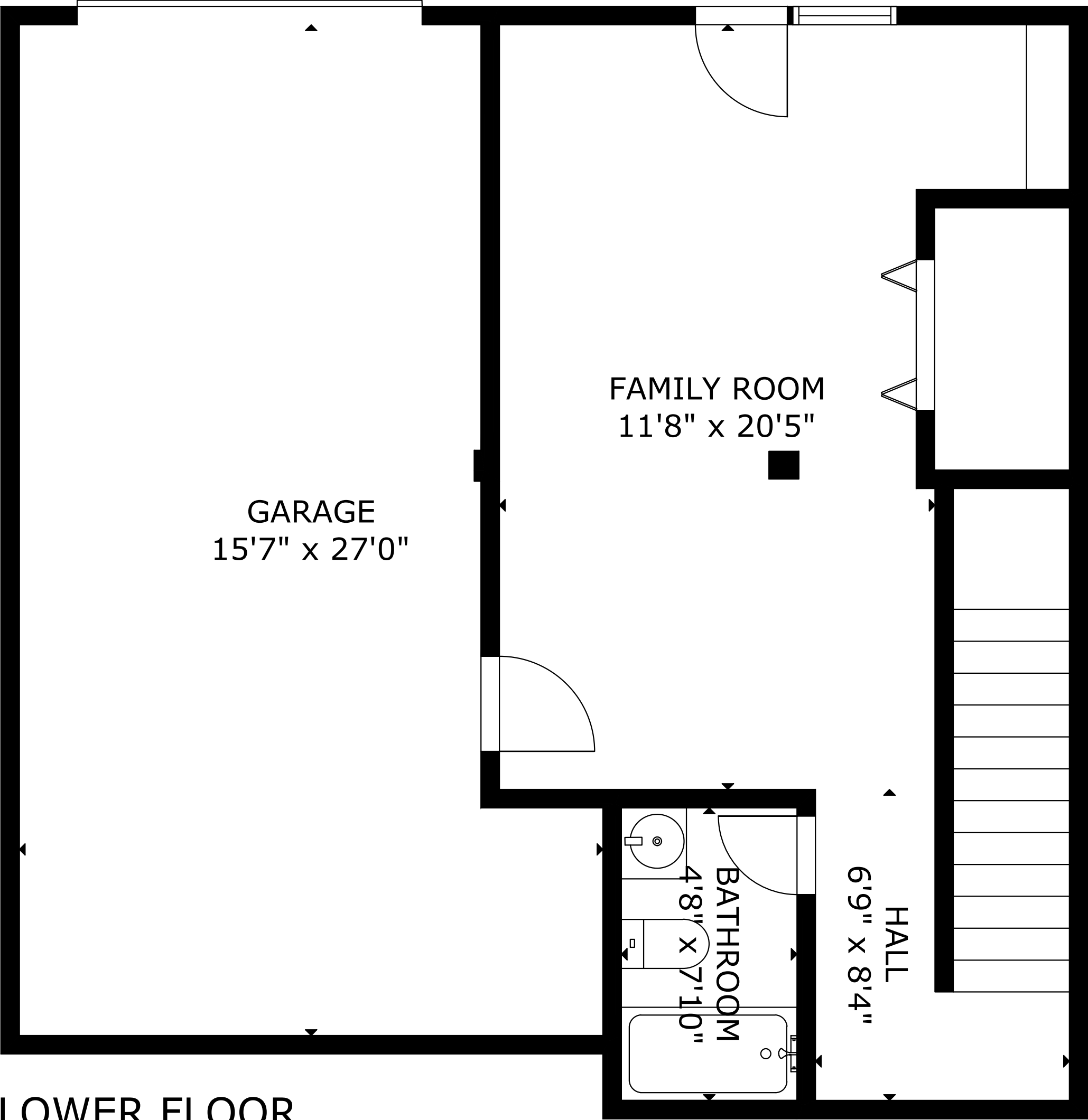
LOWER FLOOR
