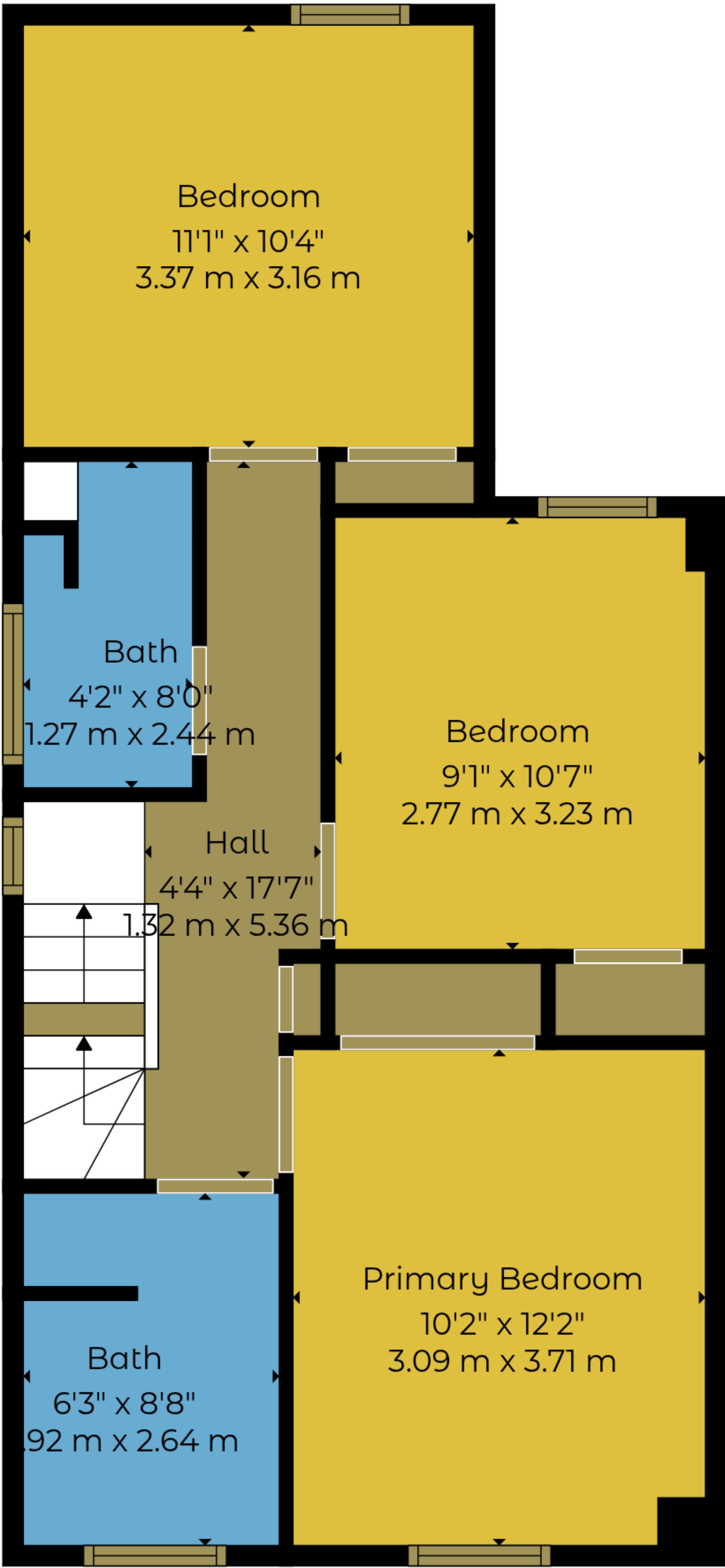
2nd Floor
