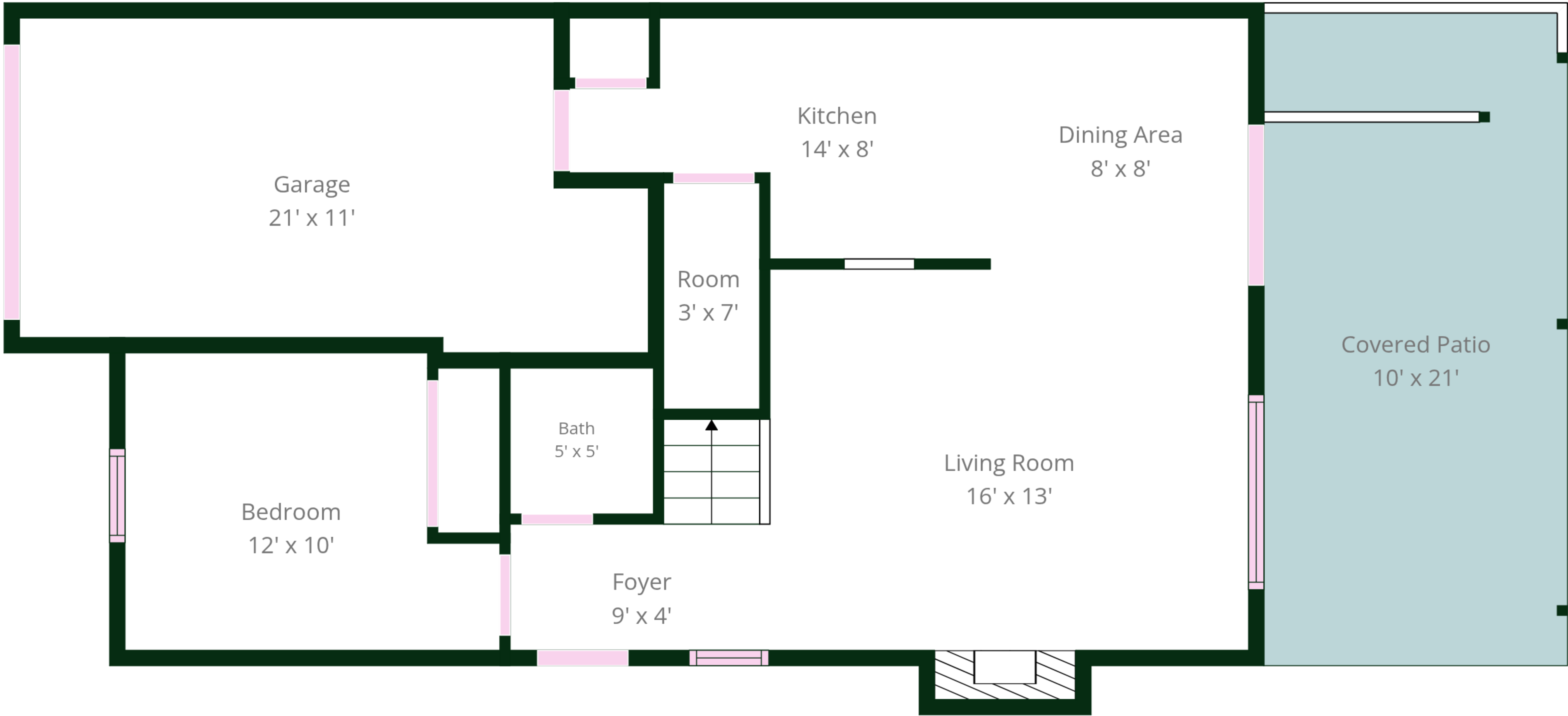
1st Floor
