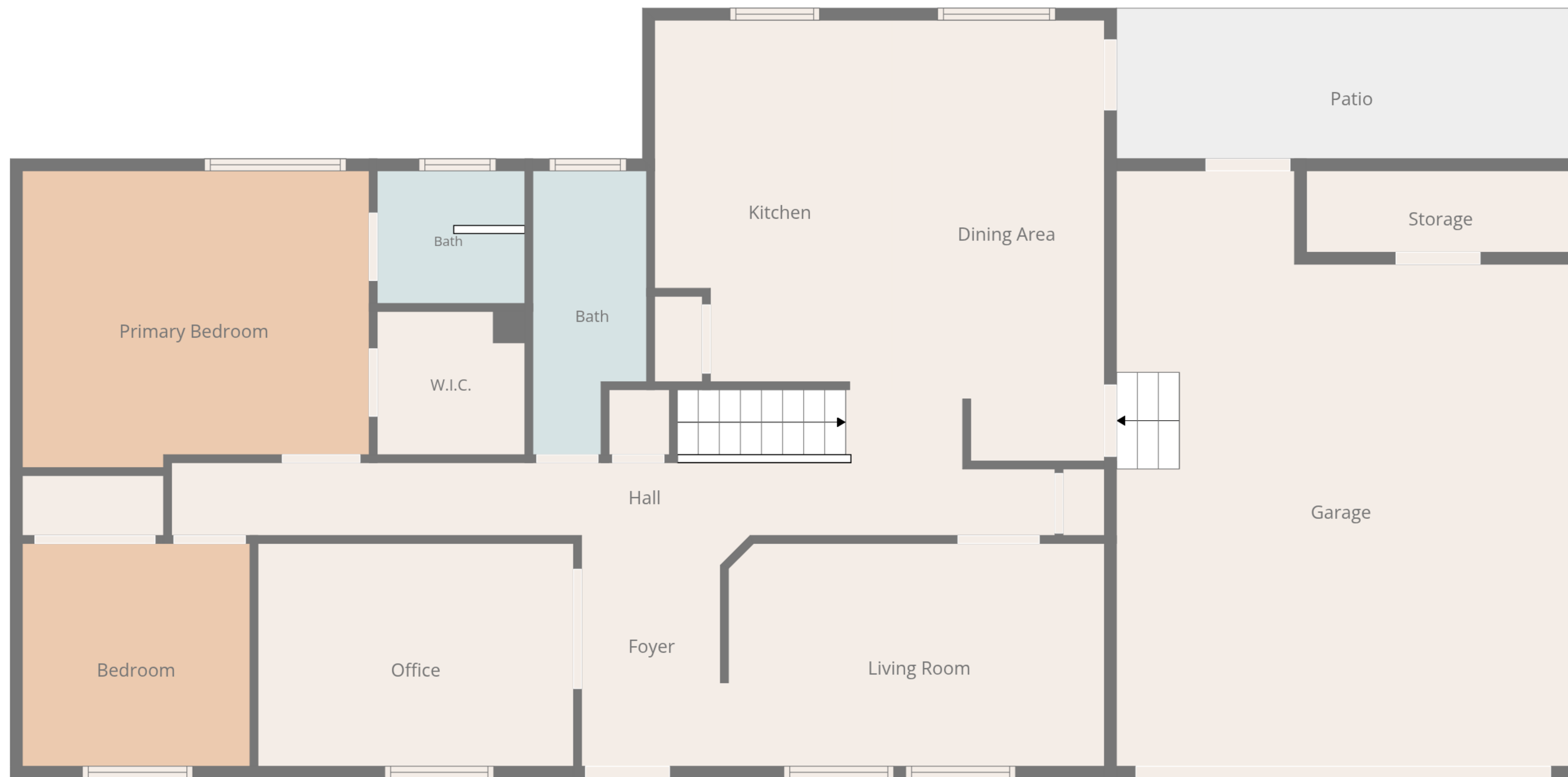
1st Floor
