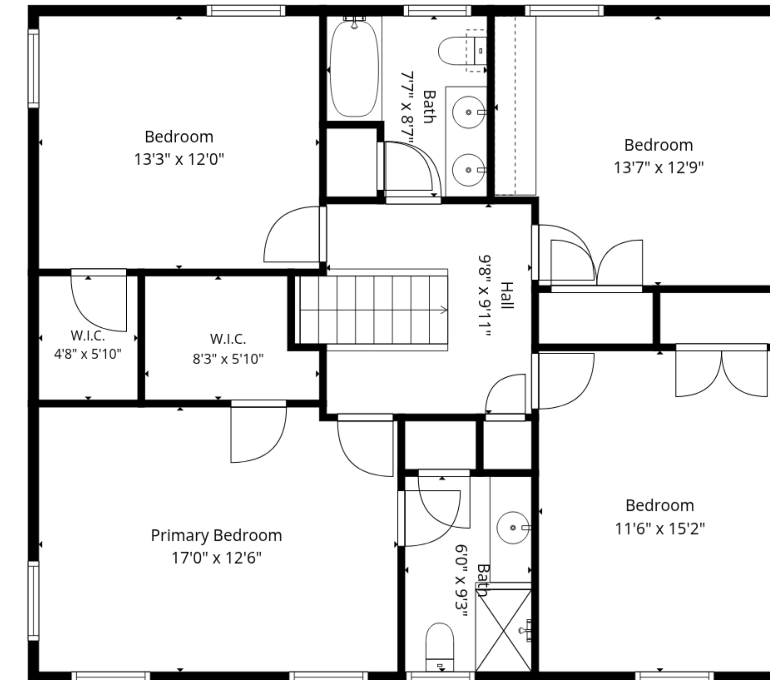
2nd Floor
