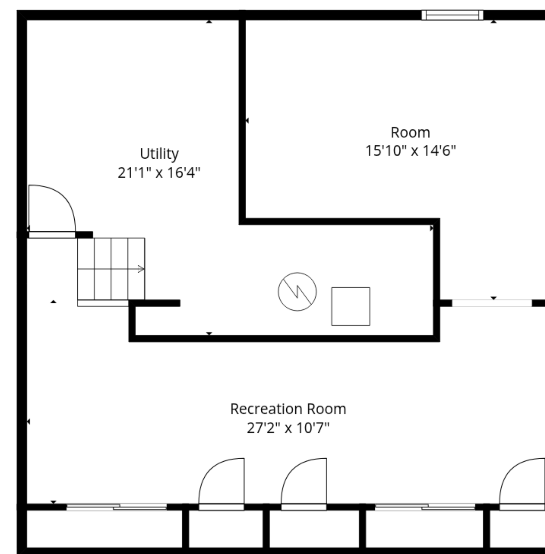
Basement
