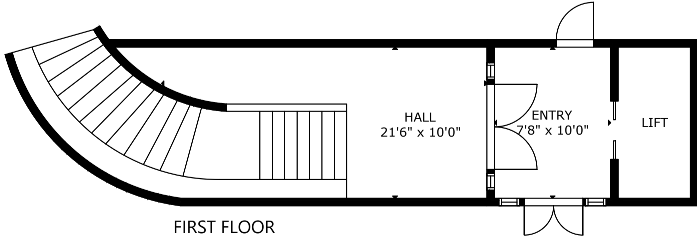
FIRST FLOOR
