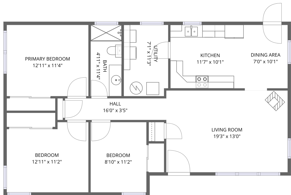
1st floor
