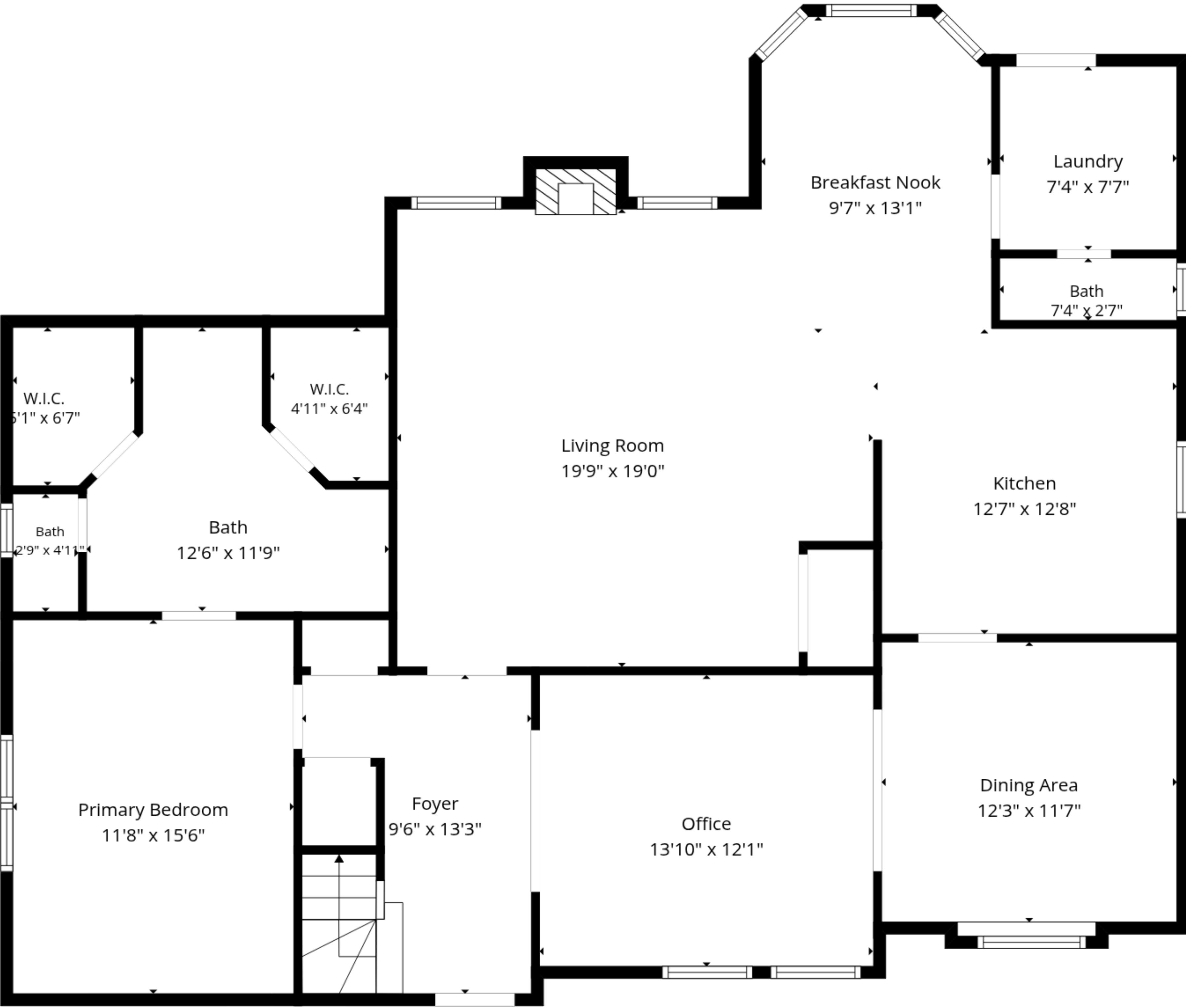
1st Floor
