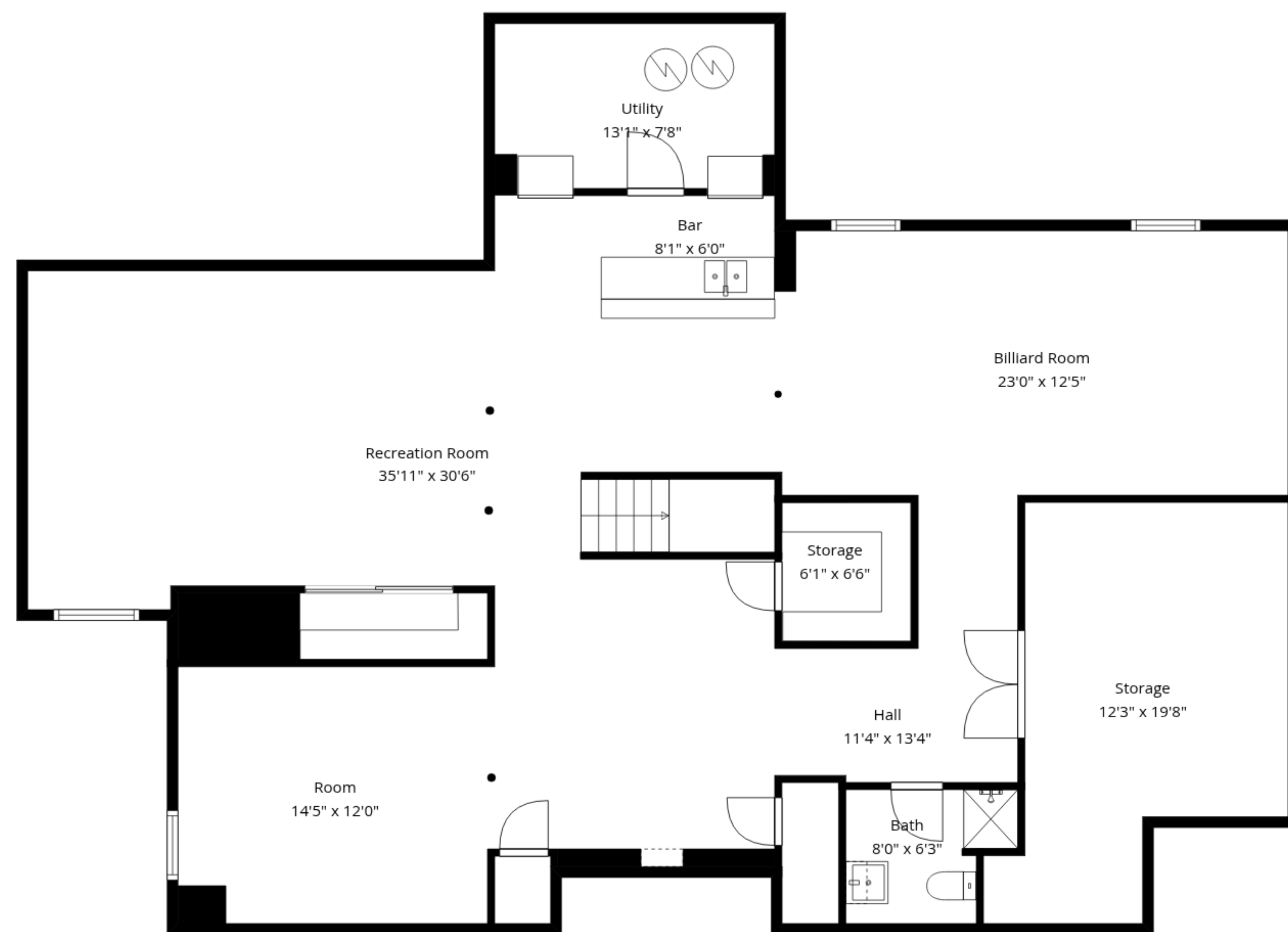
Basement
