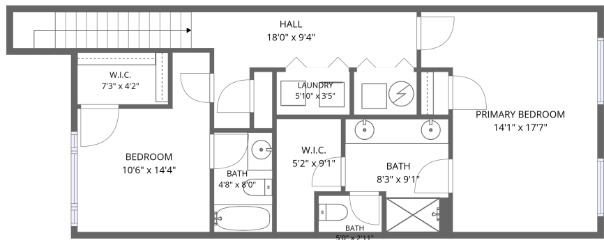
2nd floor
